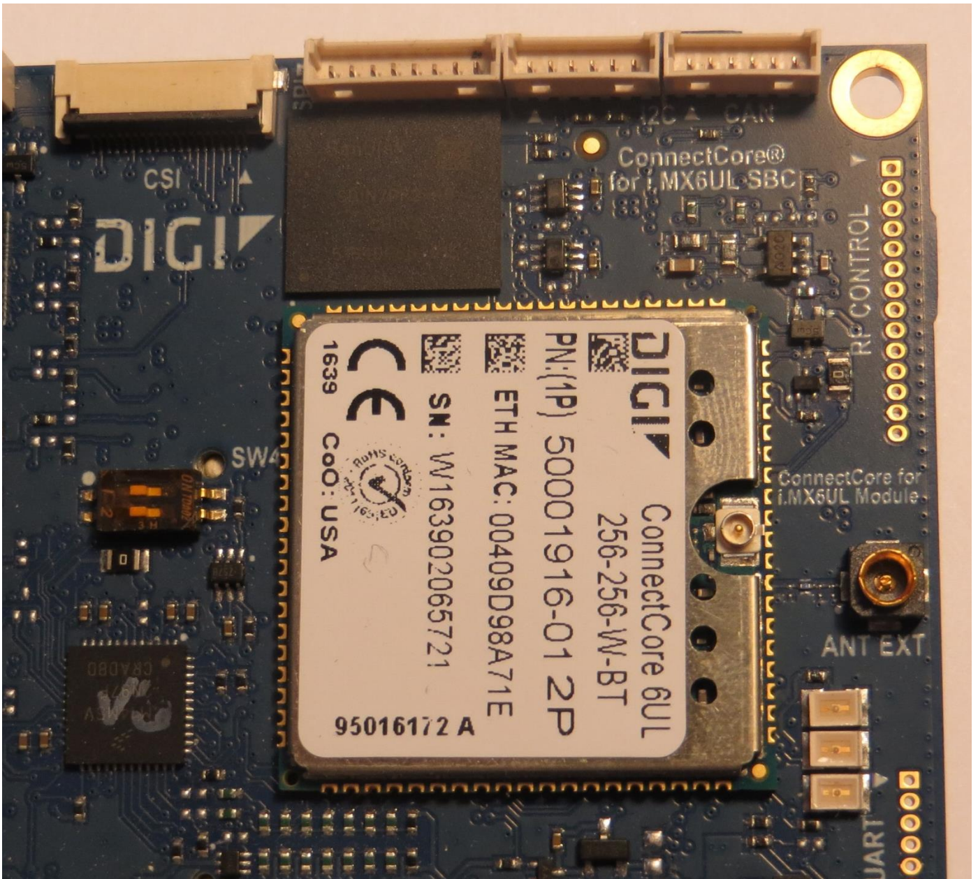
Connection between ConnectCore 6UL module and external antenna (ANT EXT)
