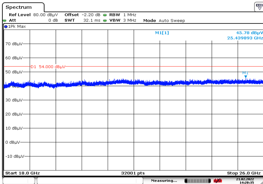
Plot 4: 18 GHz to 26 GHz, TX mode, valid for all channels, vertical & horizontal polarization, 1 Msp/s
