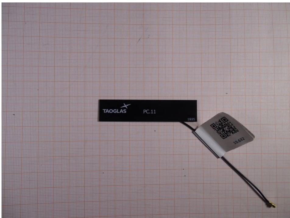
Photo 6: TAOGLAS PC11.07.0100A
