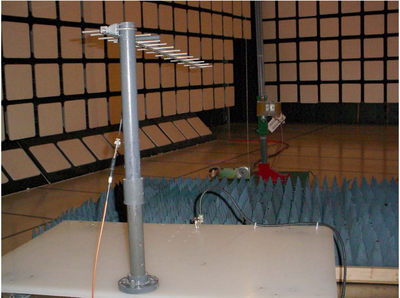
Radiated Emissions at 3 m EUT with 15.1 dBi Yagi Antenna (Orthogonal Position 2)
