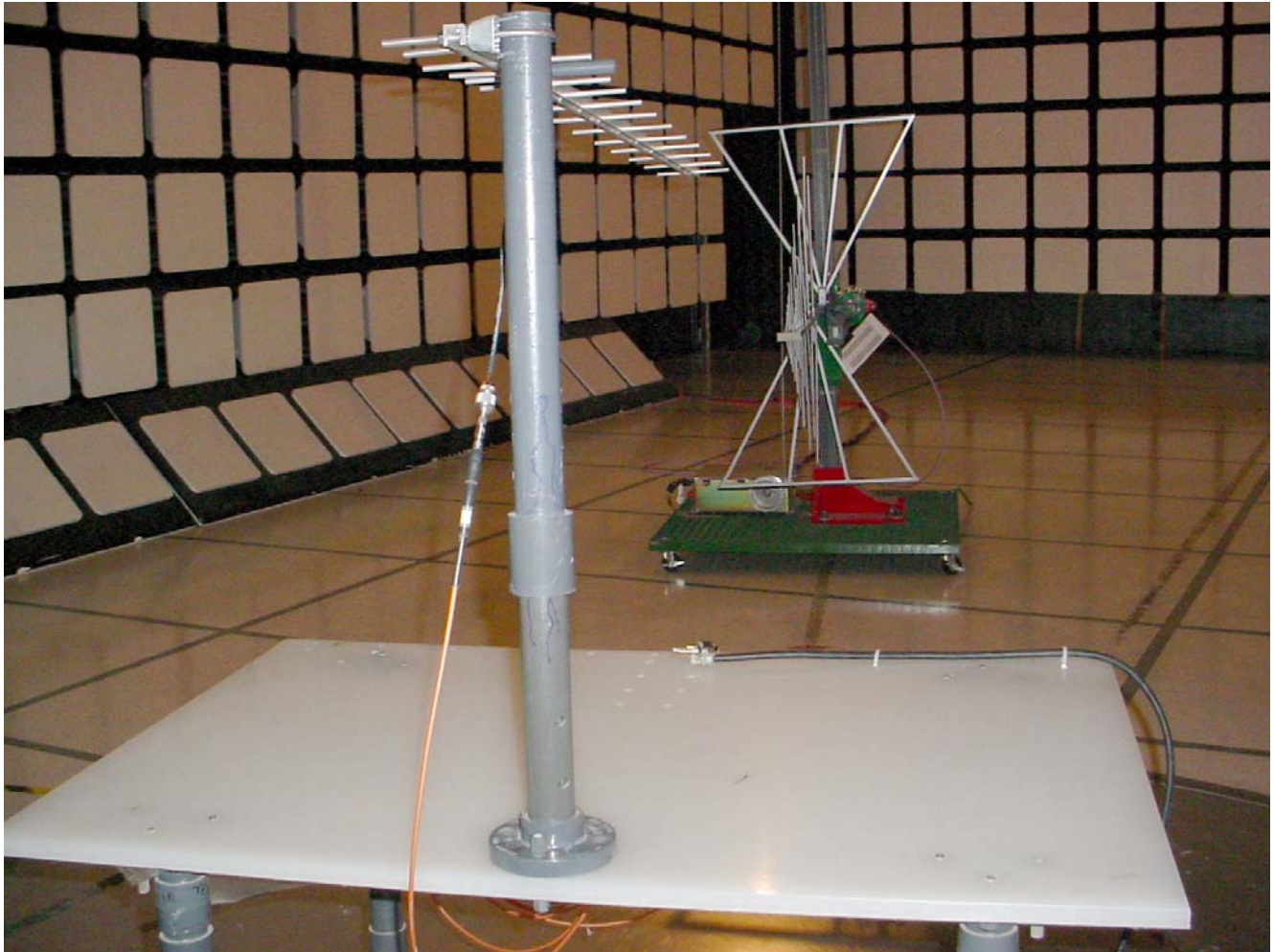
Radiated Emissions at 3 m EUT with 15.1 dBi Yagi Antenna (Orthogonal Position 1)
