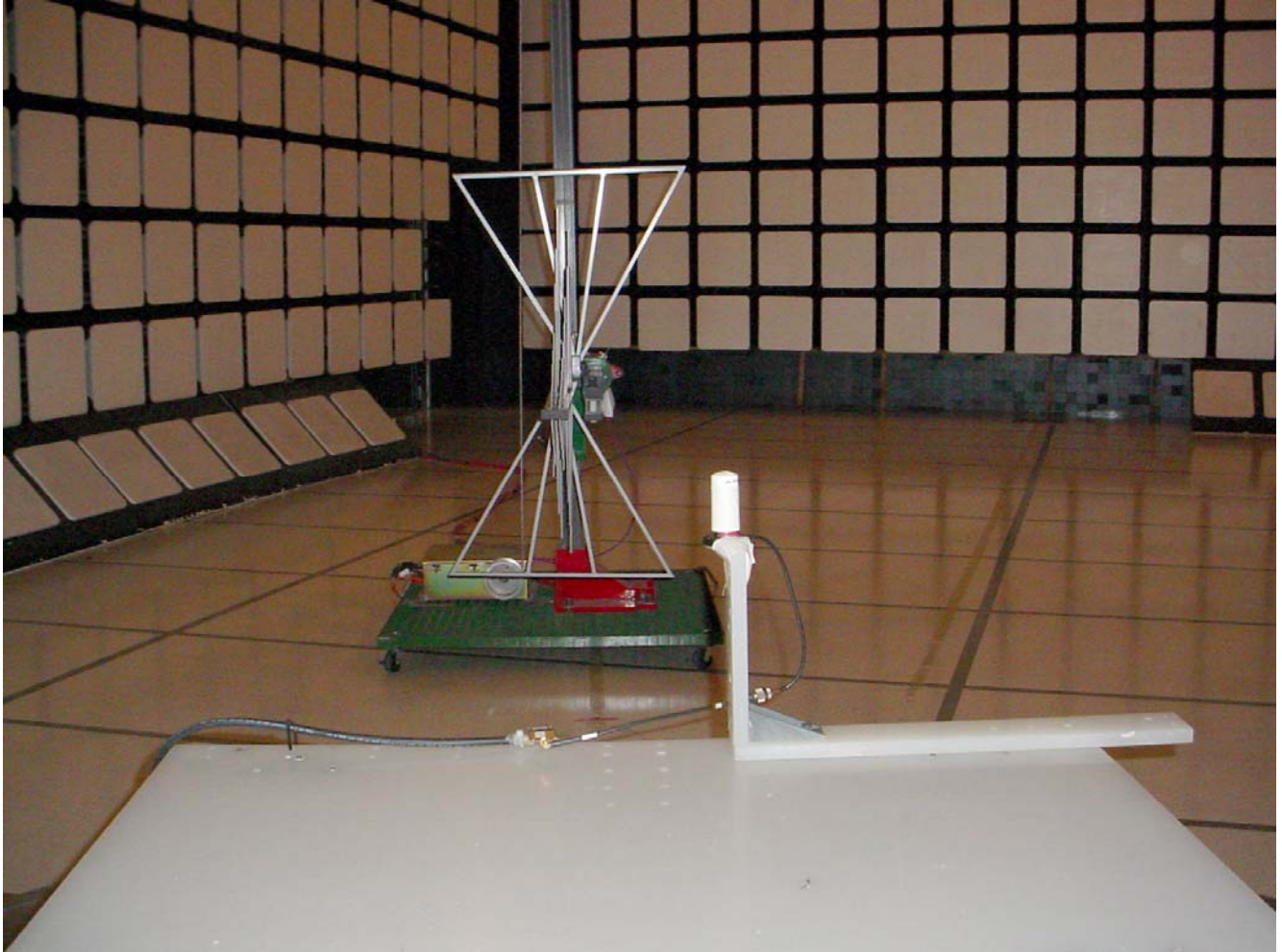
Radiated Emissions at 3 m EUT with 3.0 dBi Multi-path Antenna
