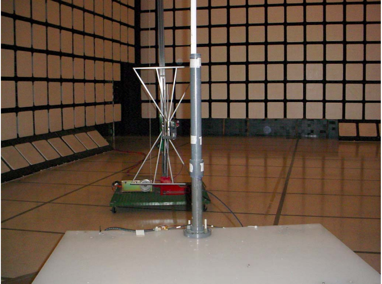
Radiated Emissions at 3 m EUT with 8.1 dBi Omni-directional Antenna
