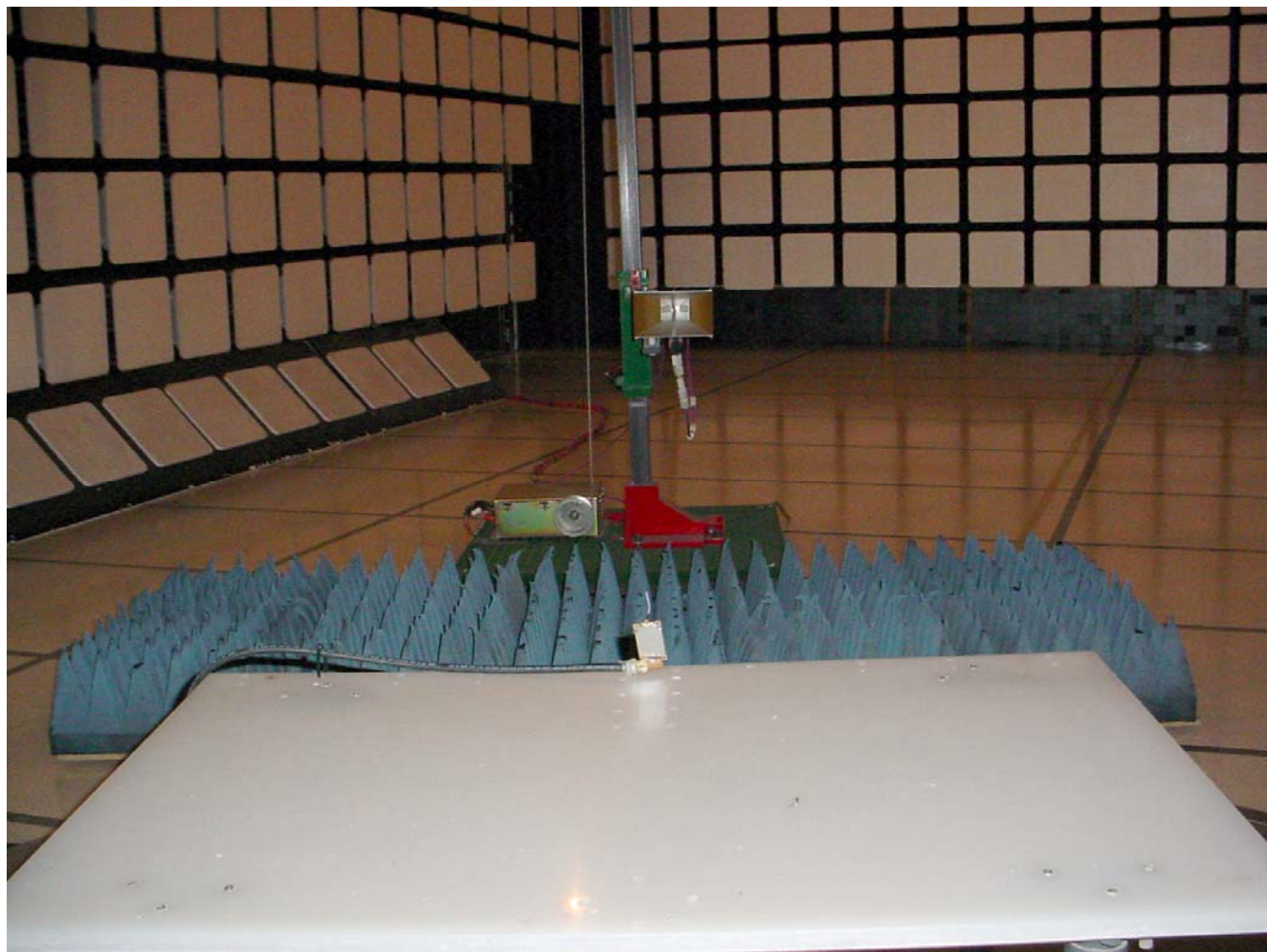
Radiated Emissions at 3 m EUT with 2.1 dBi Monopole Antenna
