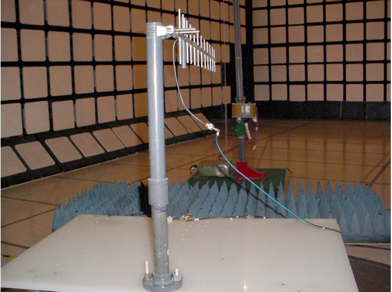
Radiated Emissions at 3 m EUT with 15.1 dBi Yagi Antenna
