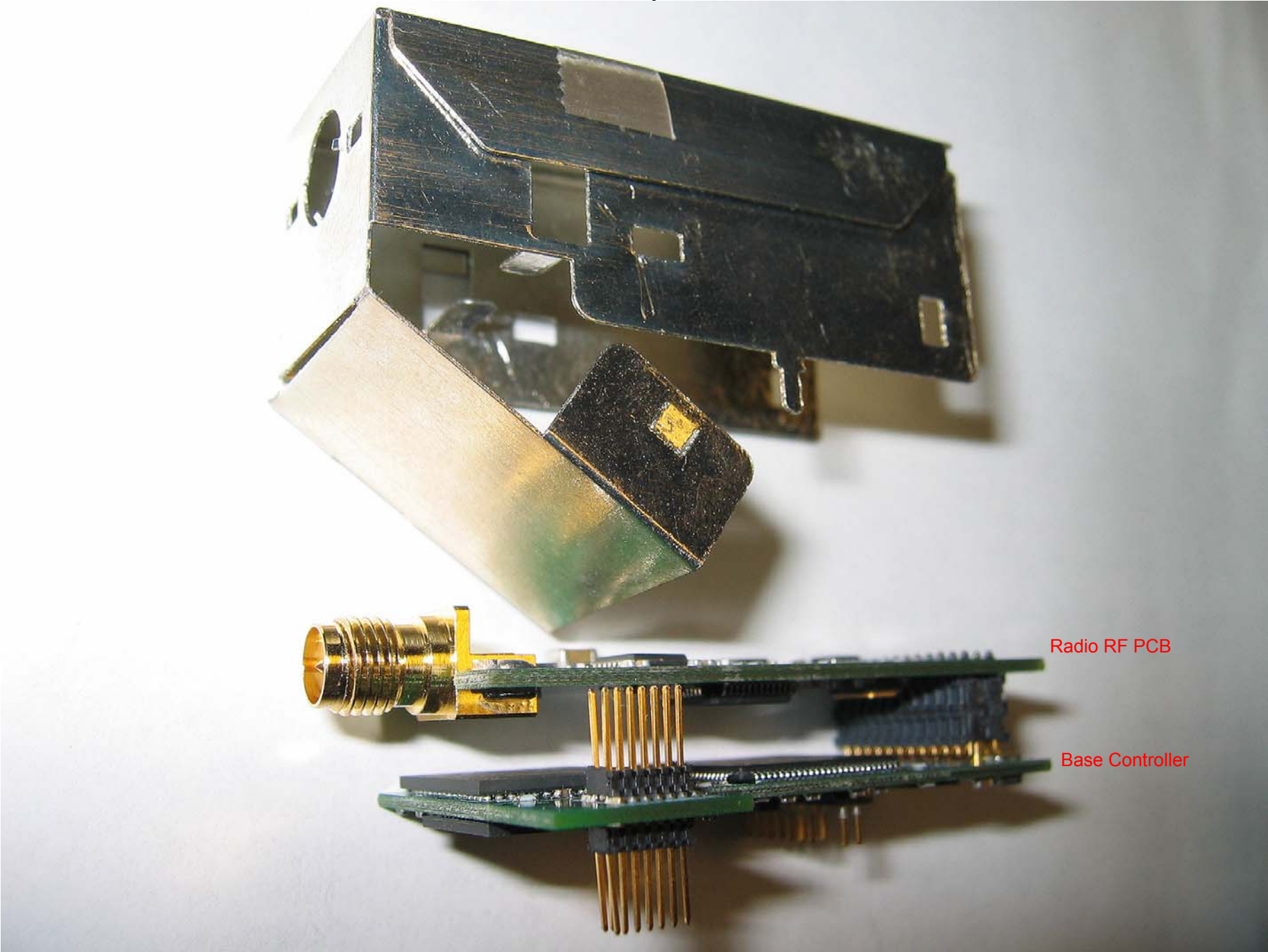
Disassembly Photo
