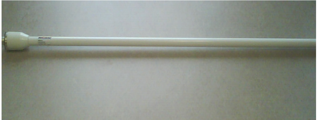
MAXRAD, MFB24010, 2.4 GHz, 10 dBi Fiberglass OMNI antenna
