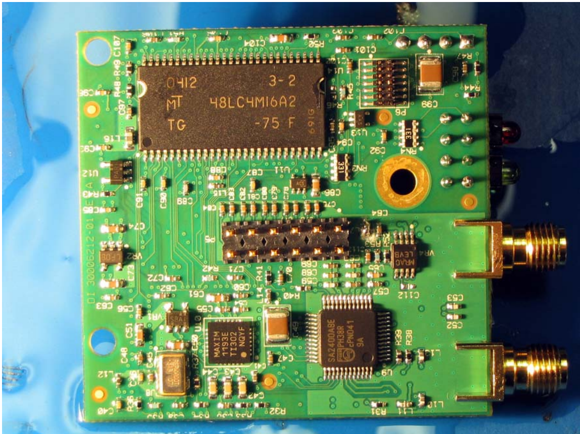
Wi-EM - Bottom View
