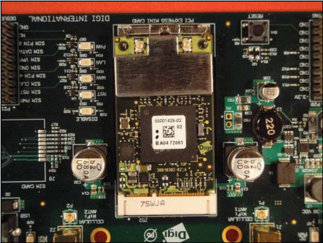
Photo 7: WLAN RF module & application / development board
