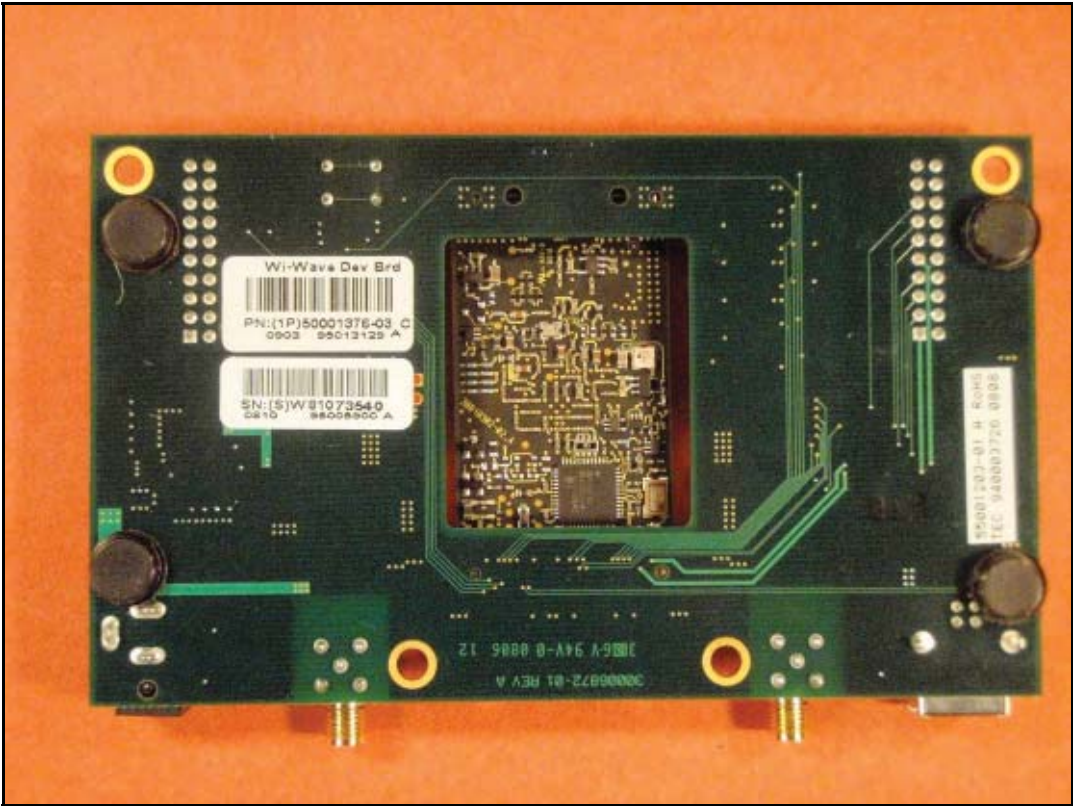
Photo 9: WLAN RF module & application / development board bottom side
