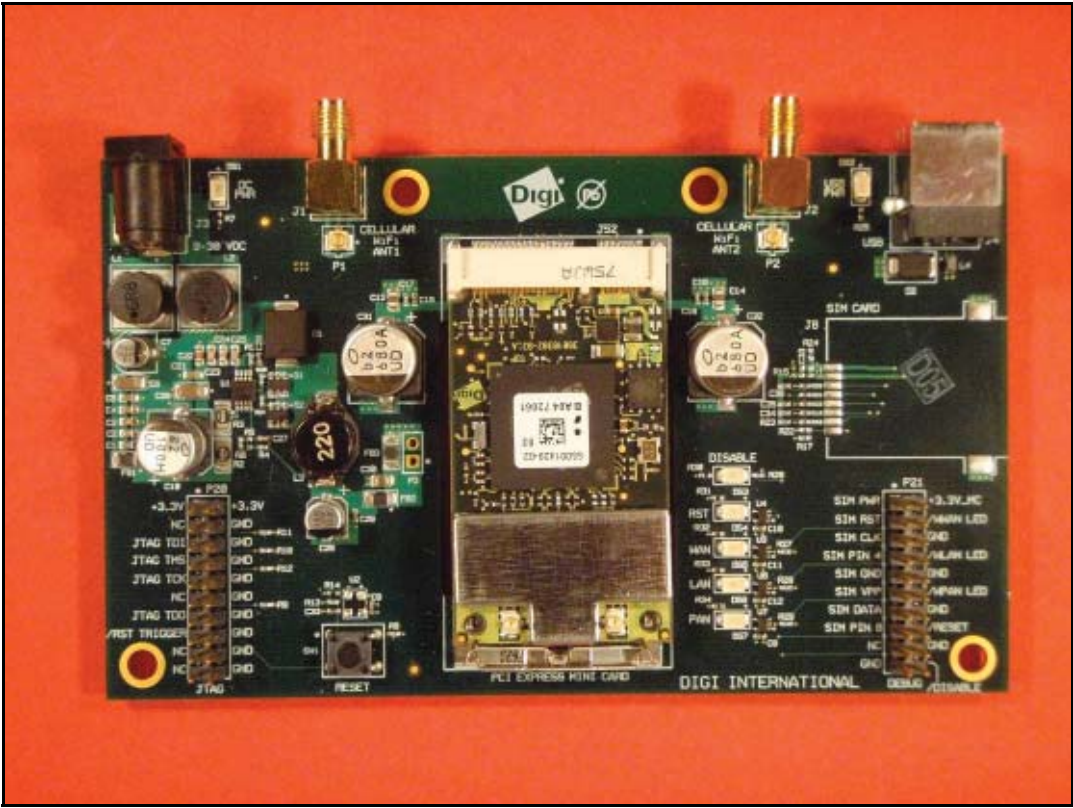
Photo 6: WLAN RF module & application / development board
