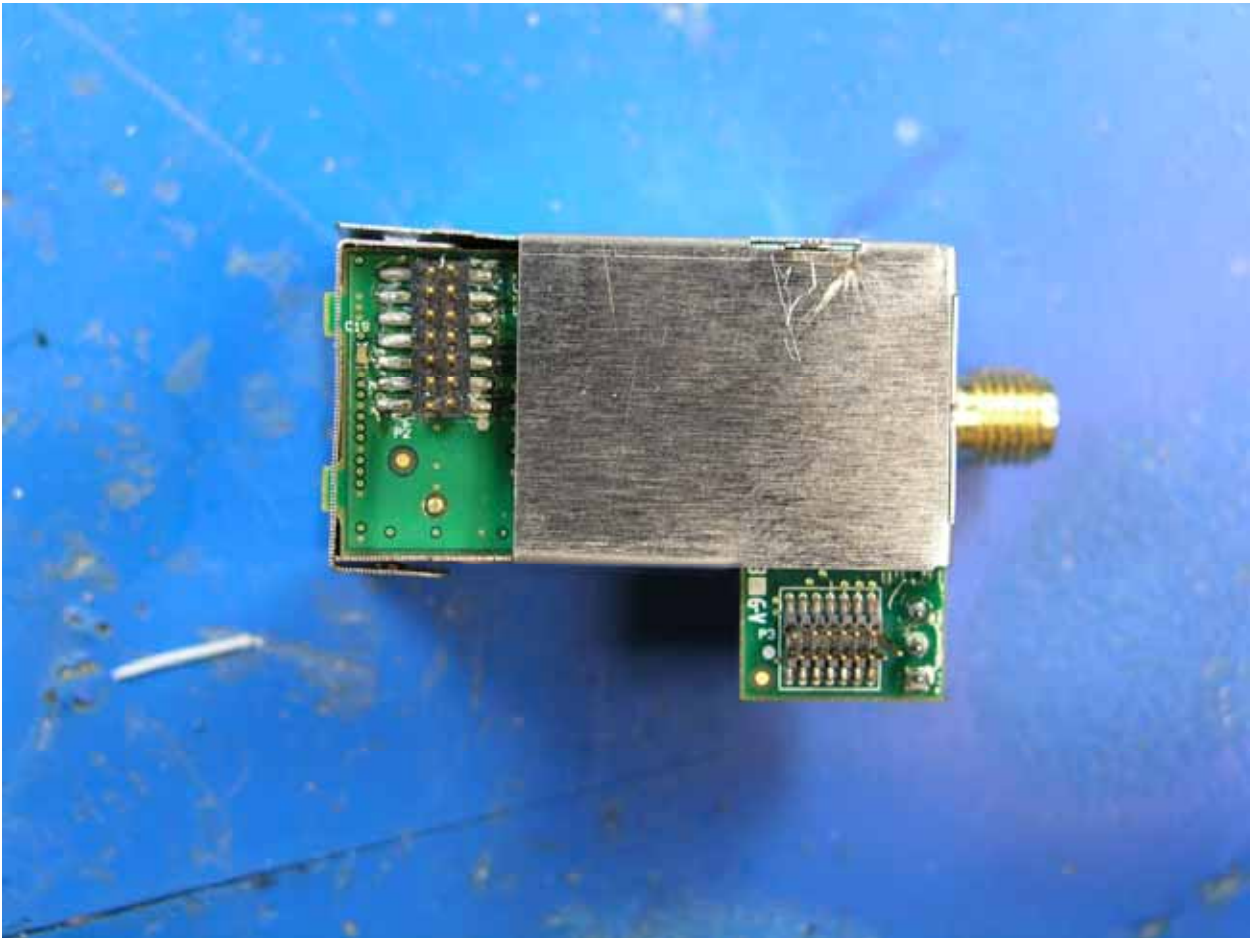
Wi-ME JTAG Bottom & User Connector View
