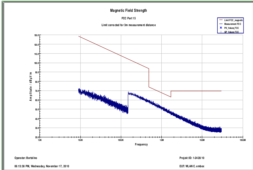
Plot 1: lowest channel; power index 35; 9 kHz to 30 MHz – magnetic
