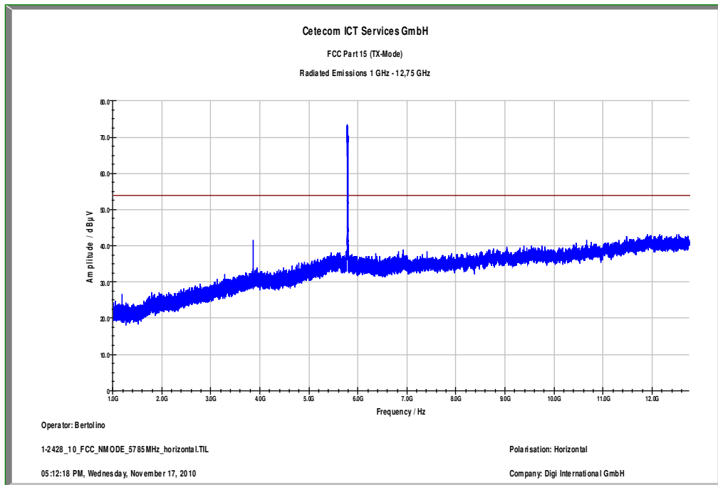
Plot 9: middle channel; power index 35; 1 GHz to 12.75 GHz – horizontal polarization
