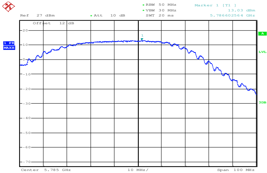
Plot 5: OFDM – mode; middle channel – 5785 MHz; power index 35; 24 MBit/s
