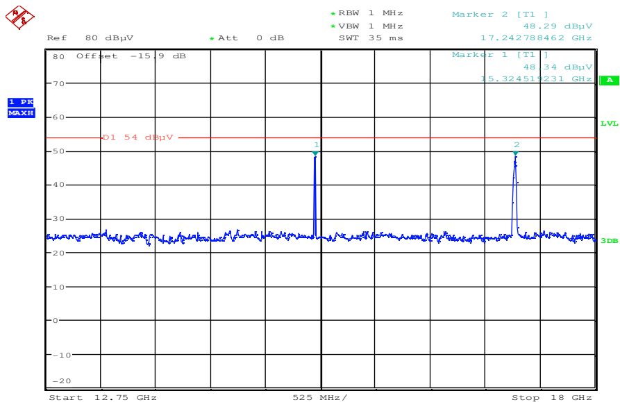
Plot 4: lowest channel; power index 35; 12.75 GHz to 18 GHz – vertical & horizontal polarization
