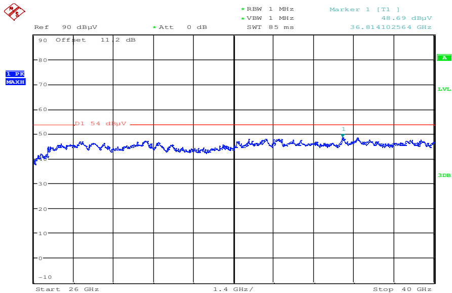
Plot 18: highest channel; power index 35; 26 GHz to 40 GHz – vertical & horizontal polarization
