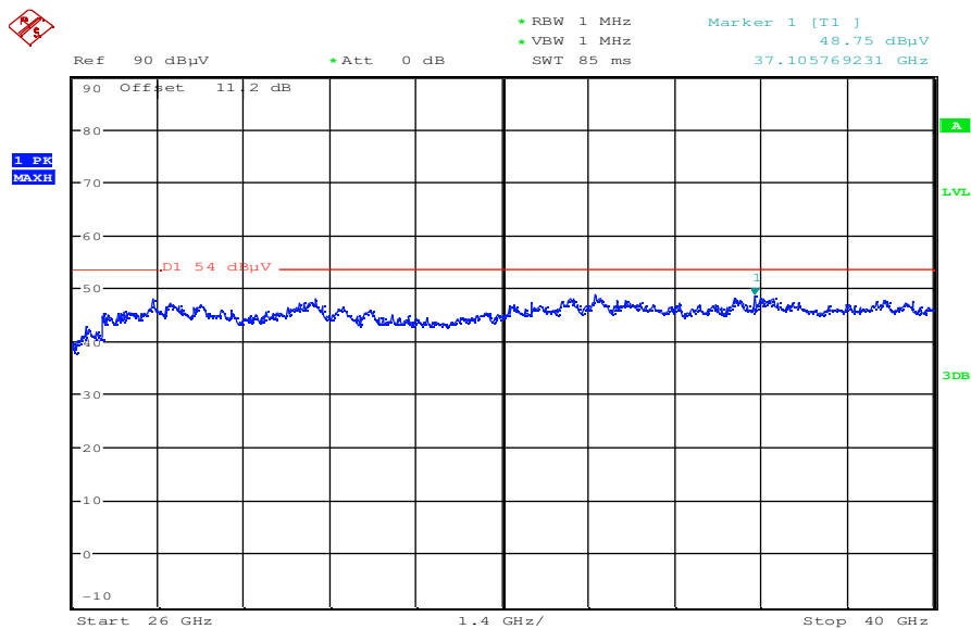
Plot 6: lowest channel; power index 35; 26 GHz to 40 GHz – vertical & horizontal polarization
