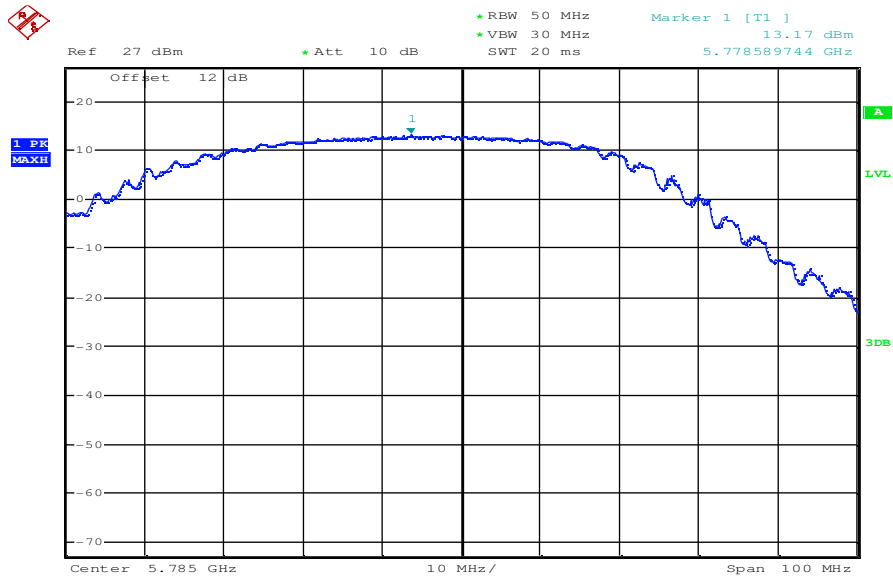
Plot 6: OFDM – mode; middle channel – 5785 MHz; power index 35; mcs5
