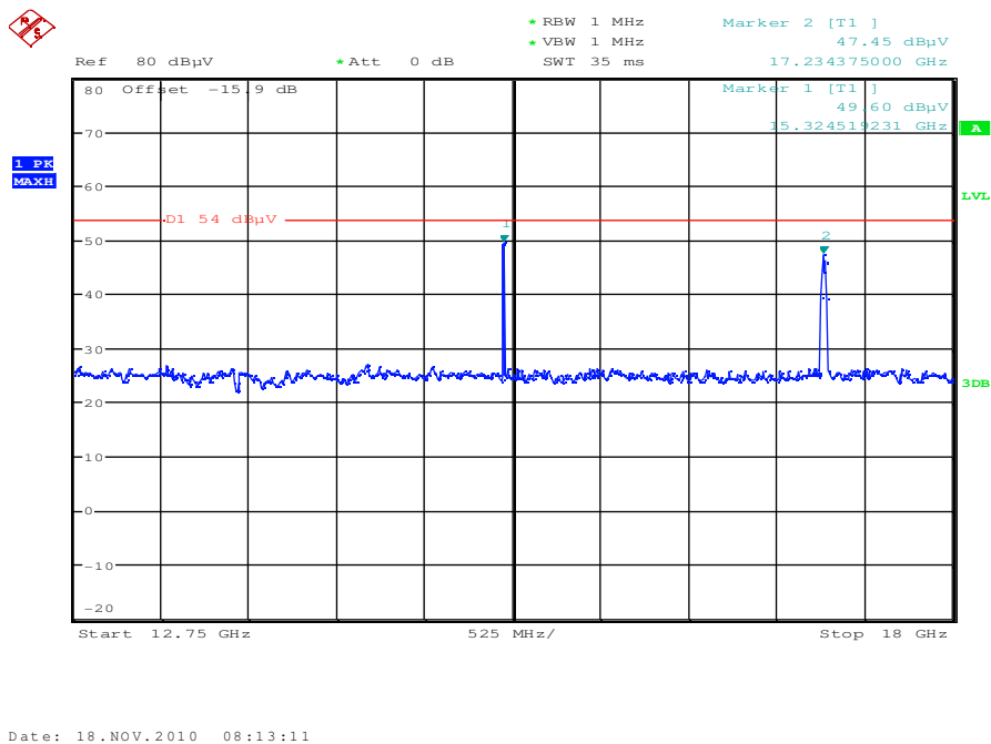
Plot 4: lowest channel; power index 35; 12.75 GHz to 18 GHz – vertical & horizontal polarization
