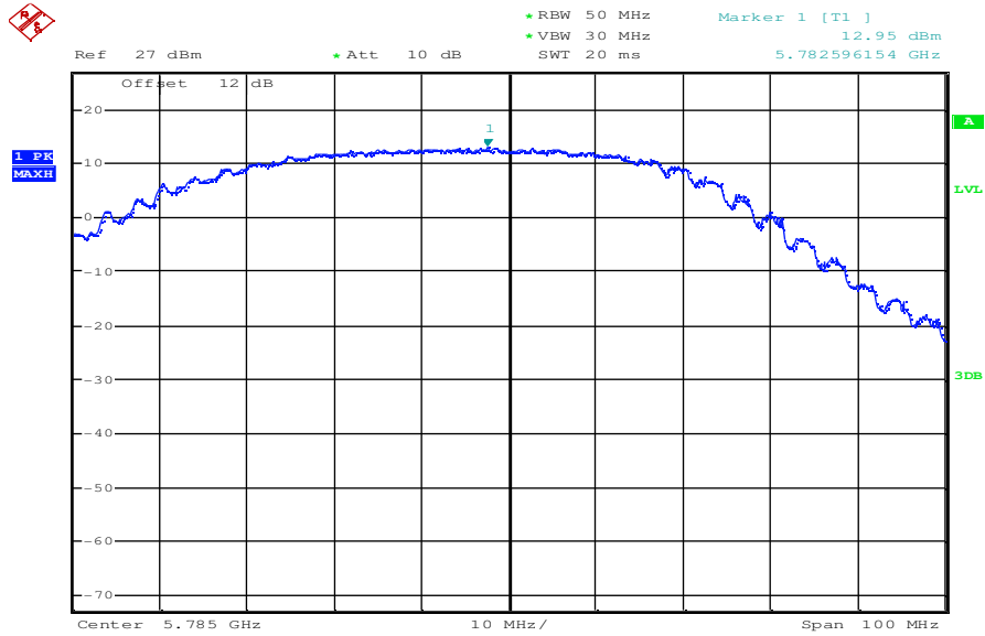
Plot 5: OFDM – mode; middle channel – 5785 MHz; power index 35; mcs4
