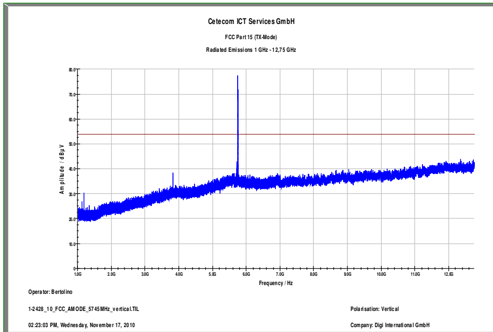
Plot 2: lowest channel; power index 35; 1 GHz to 12.75 GHz – vertical polarization
