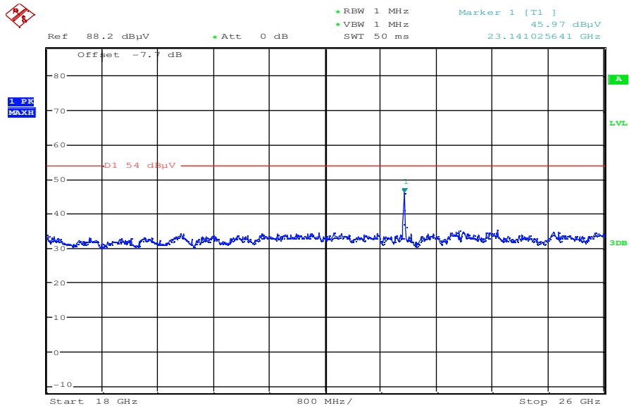
Plot 11: middle channel; power index 35; 18 GHz to 26 GHz – vertical & horizontal polarization
