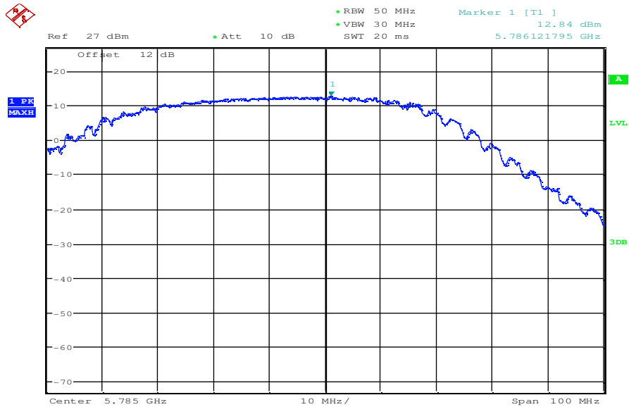
Plot 2: OFDM – mode; middle channel – 5785 MHz; power index 35; 9 MBit/s
