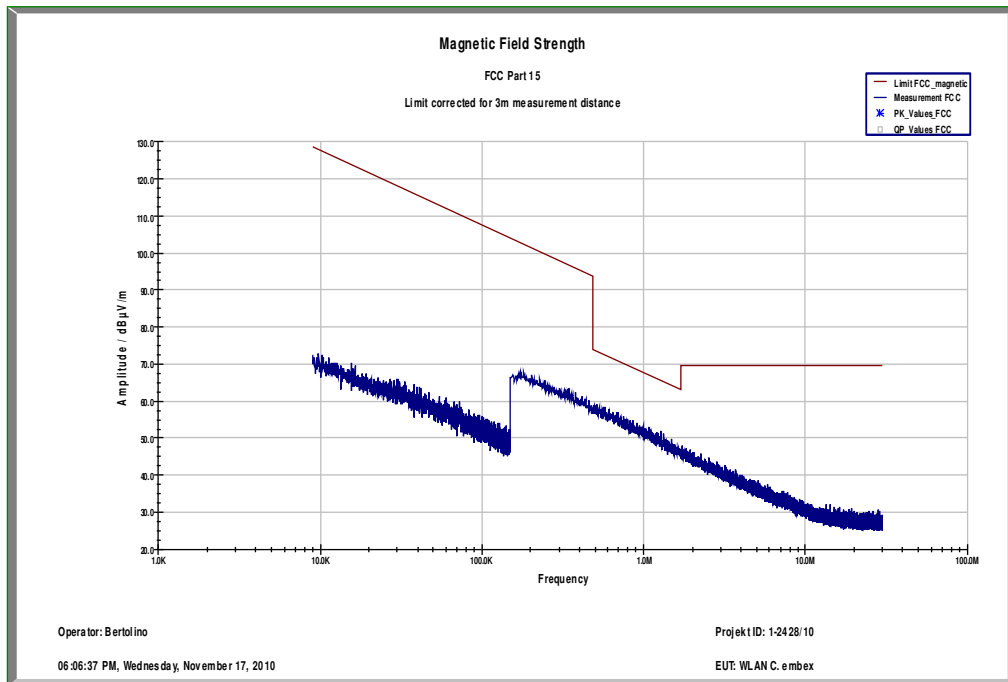
Plot 2: middle channel; power index 35; 9 kHz to 30 MHz – magnetic
