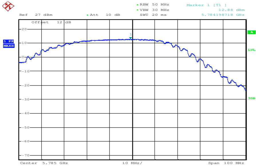
Plot 7: OFDM – mode; middle channel – 5785 MHz; power index 35; 48 MBit/s
