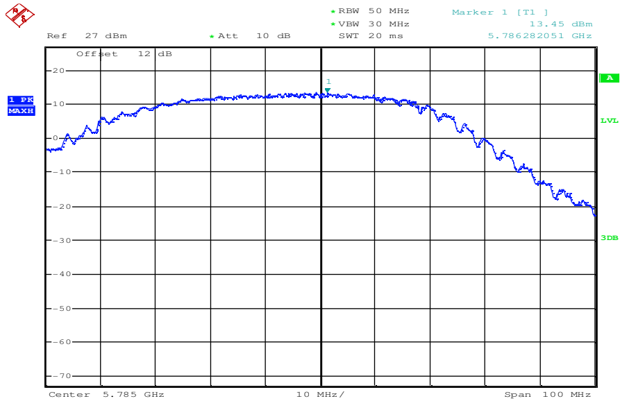
Plot 8: OFDM – mode; middle channel – 5785 MHz; power index 35; 54 MBit/s
