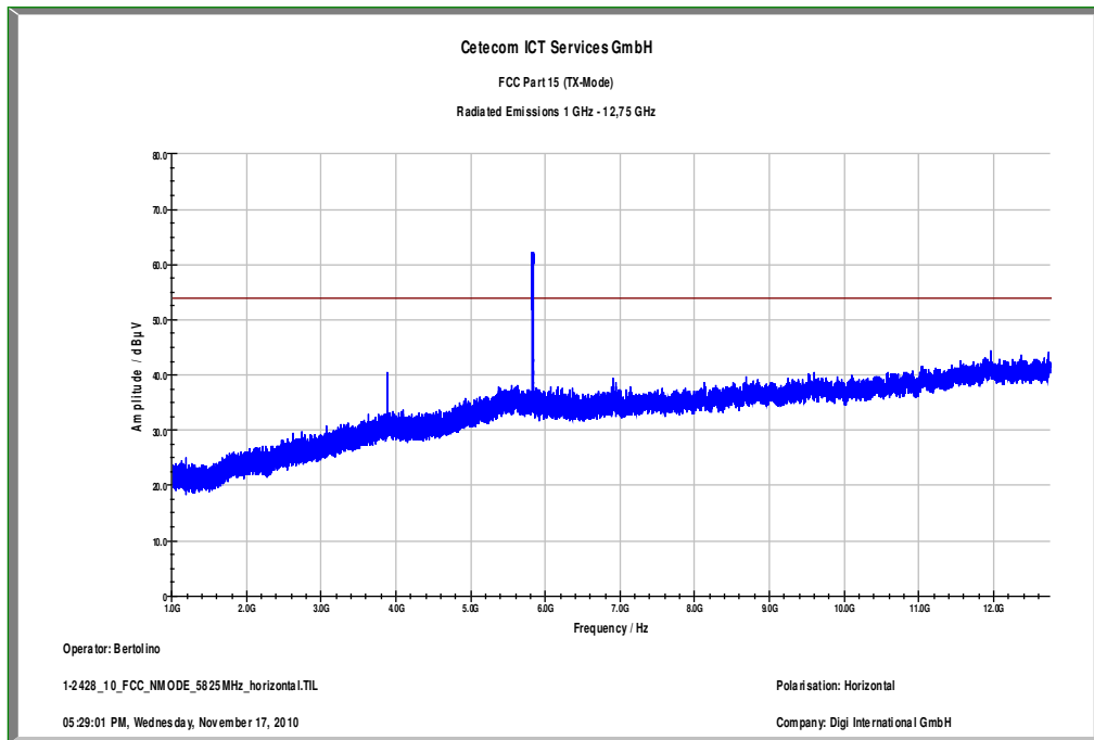
Plot 15: highest channel; power index 35; 1 GHz to 12.75 GHz – horizontal polarization
