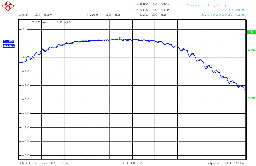
Plot 3: OFDM – mode; middle channel – 5785 MHz; power index 35; 12 MBit/s
