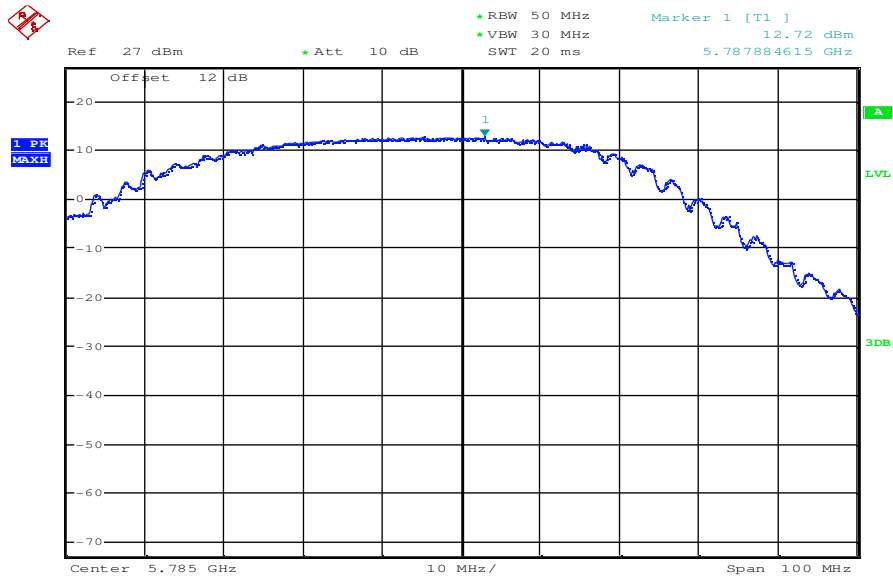
Plot 7: OFDM – mode; middle channel – 5785 MHz; power index 35; mcs6
