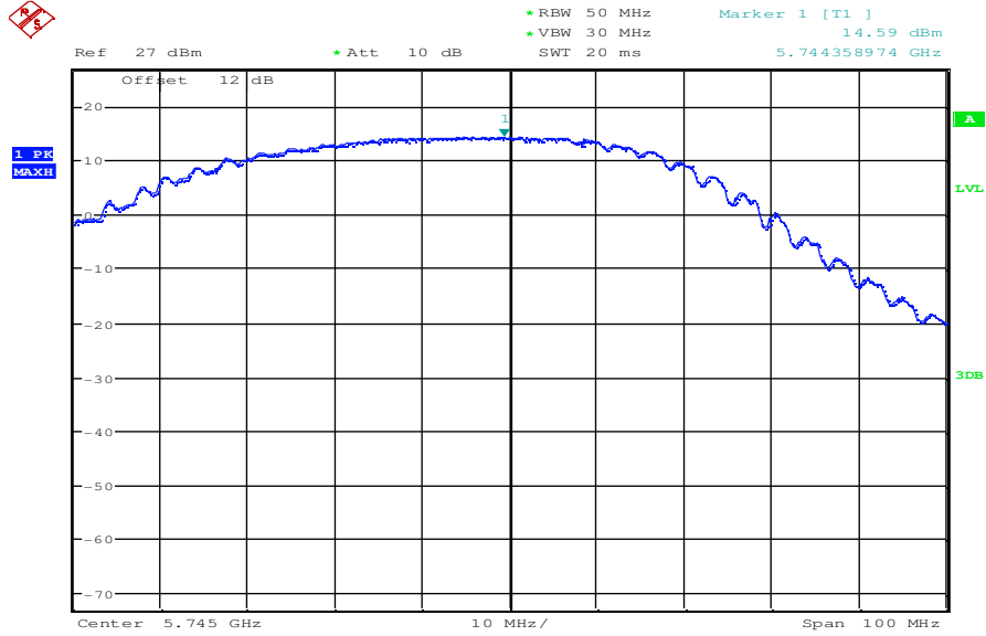
Plot 1: OFDM – mode; lowest channel – 5745 MHz; power index 35; mcs 7
