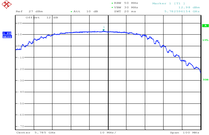
Plot 1: OFDM – mode; middle channel – 5785 MHz; power index 35; mcs0
