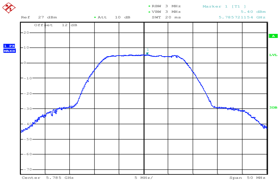
Plot 2: OFDM – mode; middle channel – 5785 MHz; power index 35; 54 MBit/s
