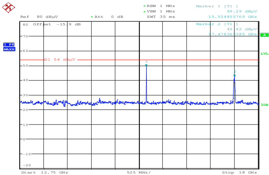
Plot 16: highest channel; power index 35; 12.75 GHz to 18 GHz – vertical & horizontal polarization
