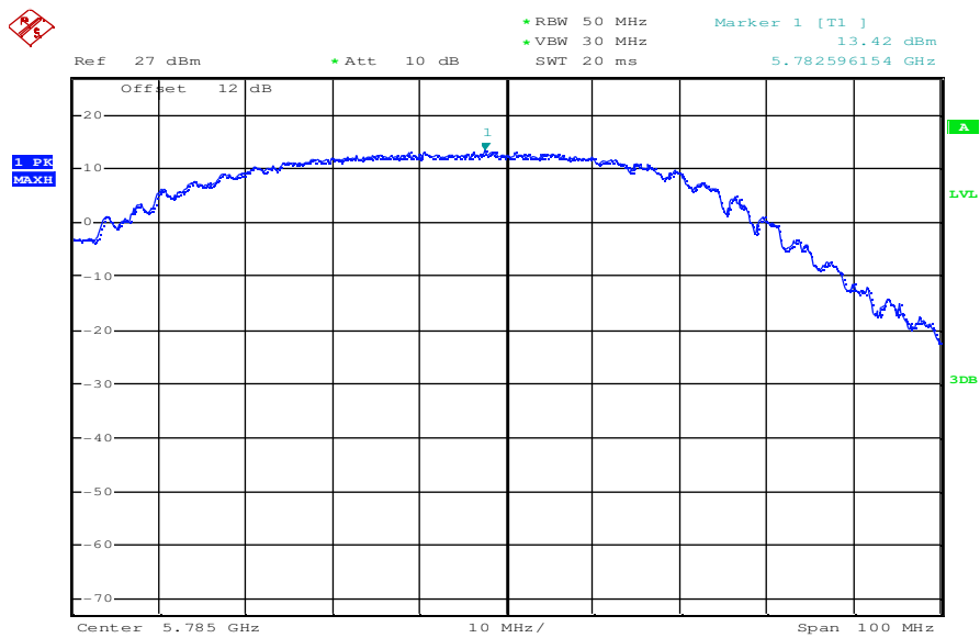
Plot 8: OFDM – mode; middle channel – 5785 MHz; power index 35; mcs7
