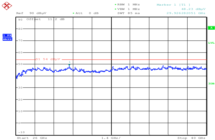
Plot 12: middle channel; power index 35; 26 GHz to 40 GHz – vertical & horizontal polarization
