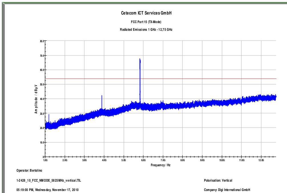
Plot 14: highest channel; power index 35; 1 GHz to 12.75 GHz – vertical polarization
