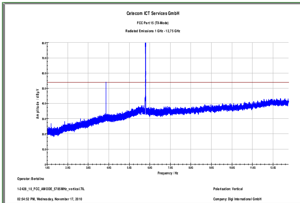
Plot 8: middle channel; power index 35; 1 GHz to 12.75 GHz – vertical polarization
