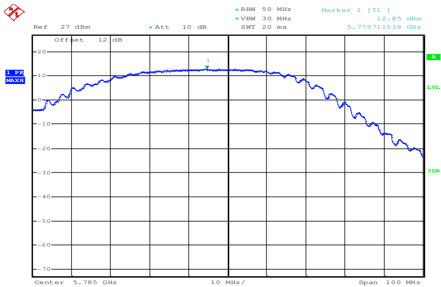
Plot 6: OFDM – mode; middle channel – 5785 MHz; power index 35; 36 MBit/s
