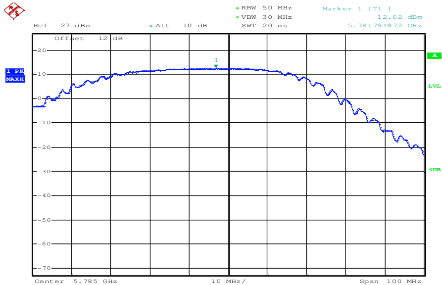
Plot 2: OFDM – mode; middle channel – 5785 MHz; power index 35; mcs1
