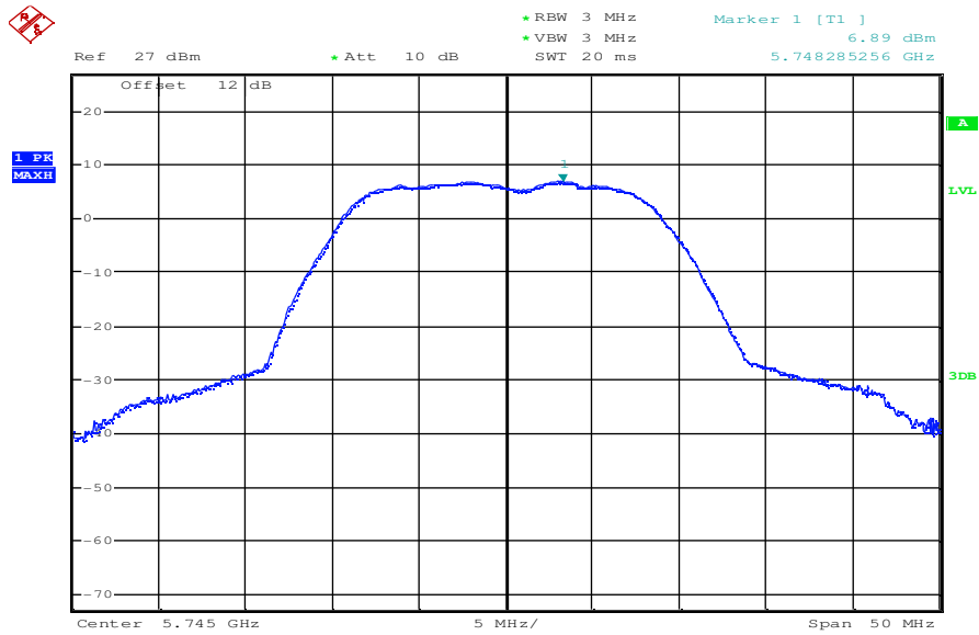
Plot 1: OFDM – mode; lowest channel – 5745 MHz; power index 35; 54 MBit/s
