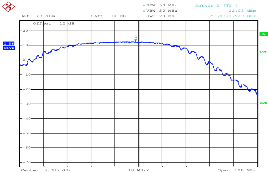
Plot 4: OFDM – mode; middle channel – 5785 MHz; power index 35; 18 MBit/s
