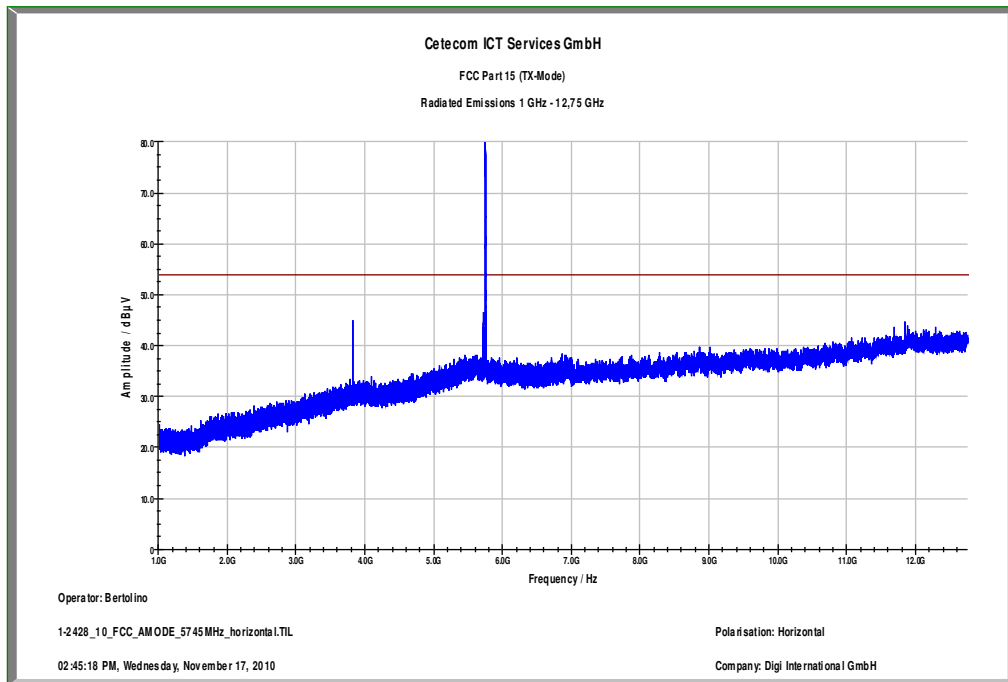
Plot 3: lowest channel; power index 35; 1 GHz to 12.75 GHz – horizontal polarization
