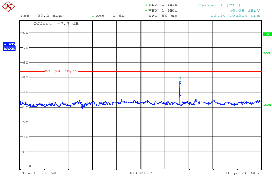
Plot 17: highest channel; power index 35; 18 GHz to 26 GHz – vertical & horizontal polarization
