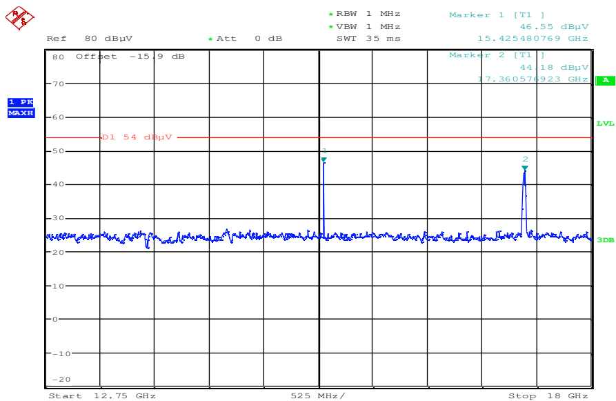
Plot 10: middle channel; power index 35; 12.75 GHz to 18 GHz – vertical & horizontal polarization
