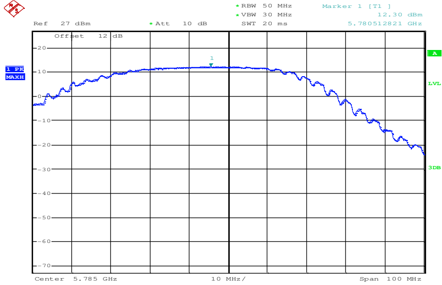
Plot 1: OFDM – mode; middle channel – 5785 MHz; power index 35; 6 MBit/s
