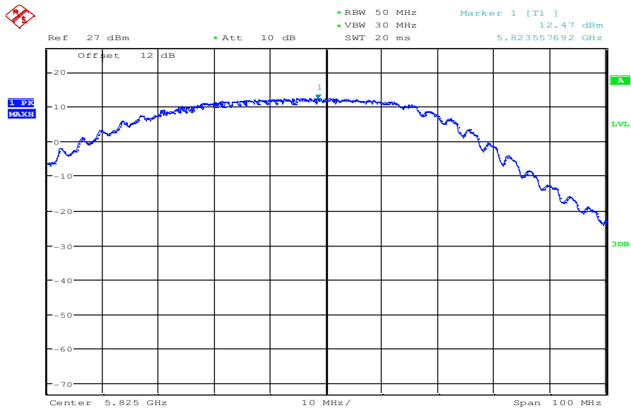
Plot 3: OFDM – mode; highest channel – 5825 MHz; power index 35; 54 MBit/s
