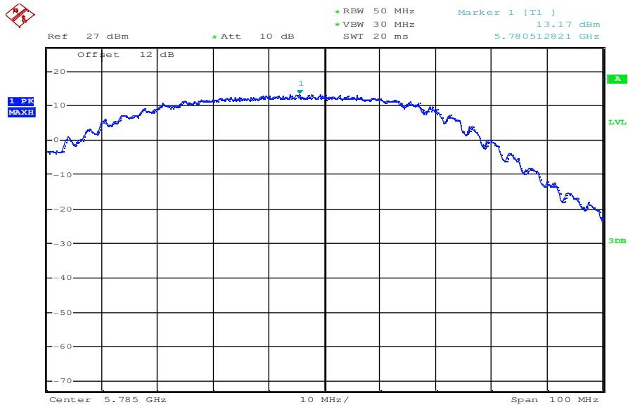
Plot 3: OFDM – mode; middle channel – 5785 MHz; power index 35; mcs2
