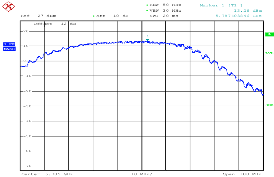
Plot 4: OFDM – mode; middle channel – 5785 MHz; power index 35; mcs3
