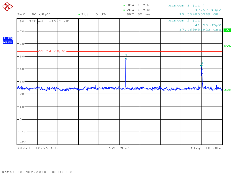
Plot 16: highest channel; power index 35; 12.75 GHz to 18 GHz – vertical & horizontal polarization
