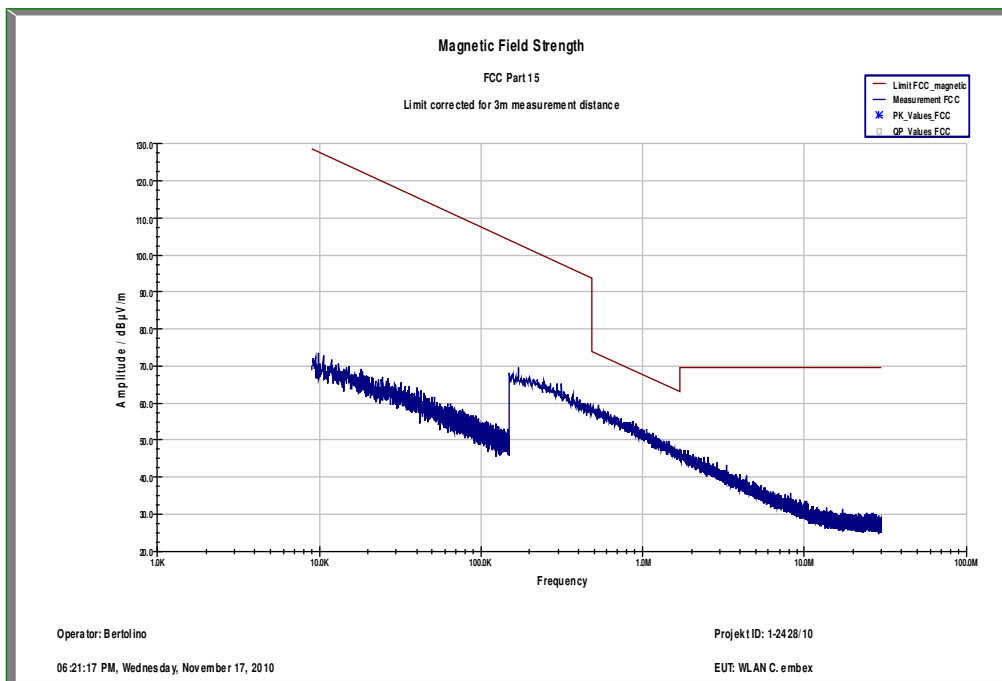
Plot 3: highest channel; power index 35; 9 kHz to 30 MHz – magnetic
