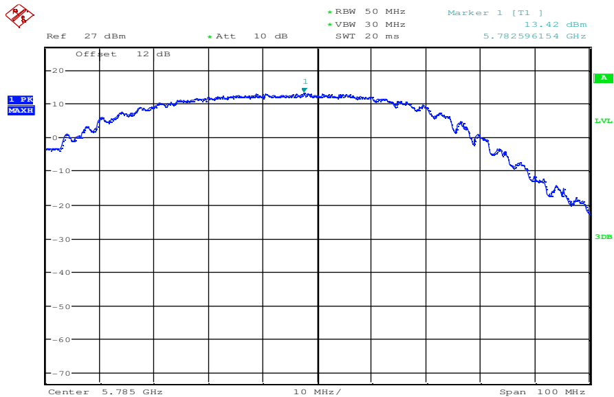
Plot 2: OFDM – mode; middle channel – 5785 MHz; power index 35; mcs 7
