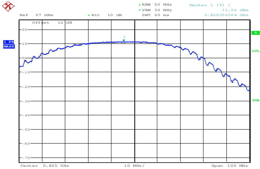
Plot 3: OFDM – mode; highest channel – 5825 MHz; power index 35; mcs 7
