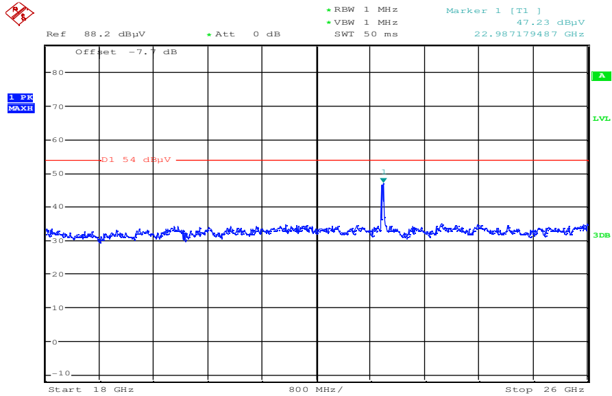
Plot 5: lowest channel; power index 35; 18 GHz to 26 GHz – vertical & horizontal polarization
