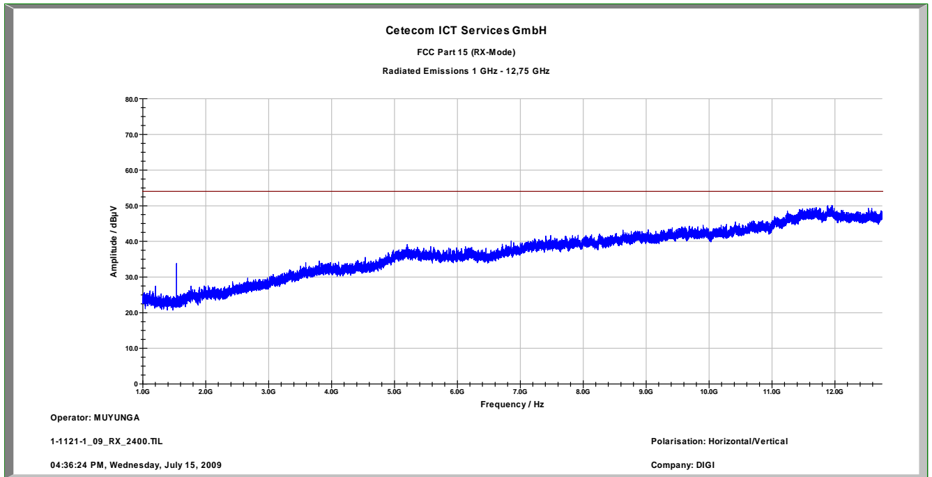
Plot 2: 1 – 12.75 GHz vertical / horizontal (receiver)
