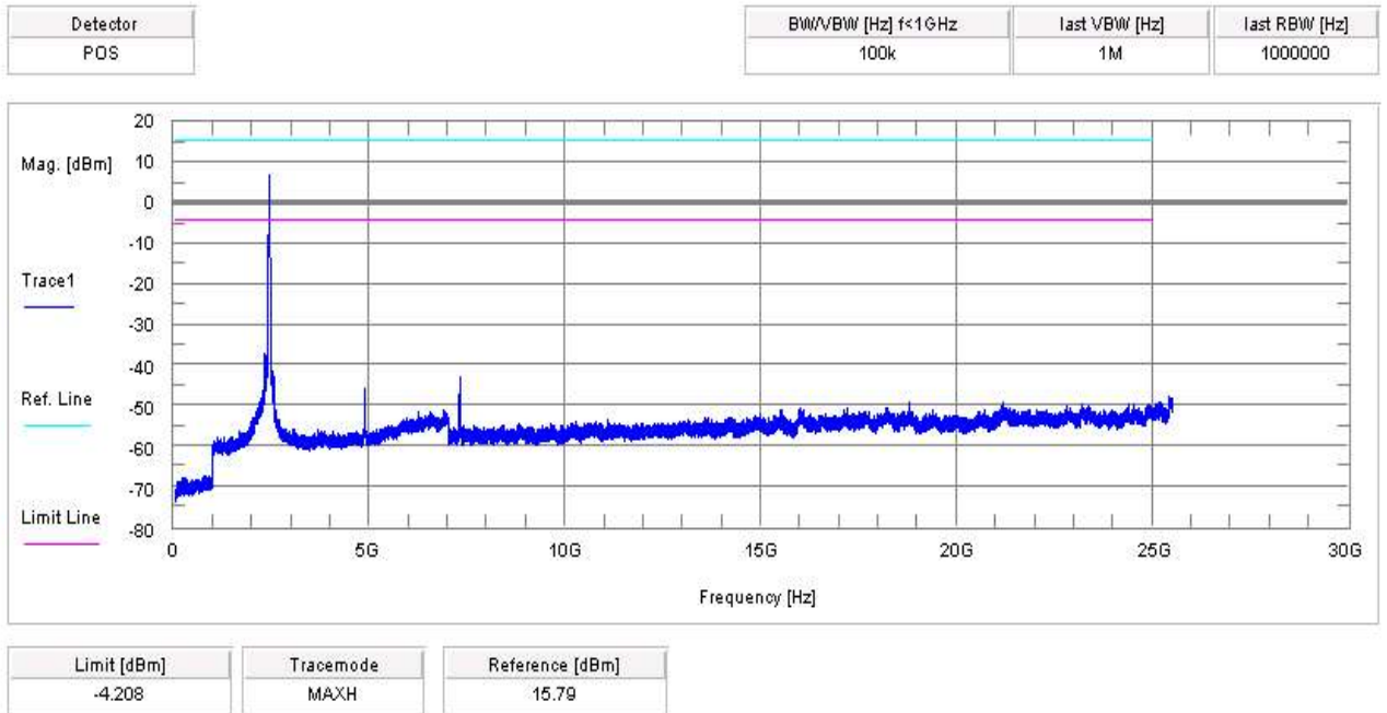
Plot 2: Middle Channel Power Index: 35
