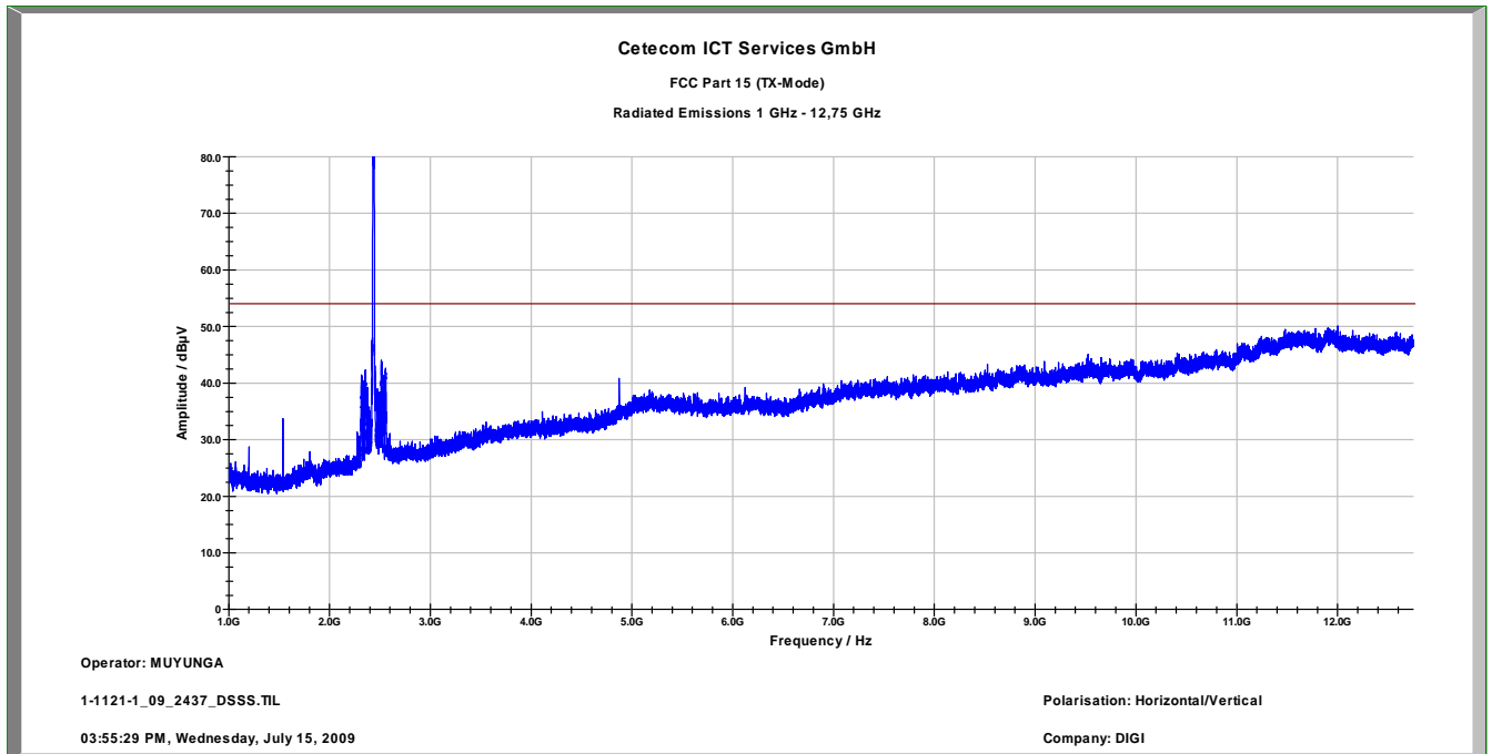
Plot 5: 1 – 12.75 GHz (middle channel) Max. Power Index: 35
