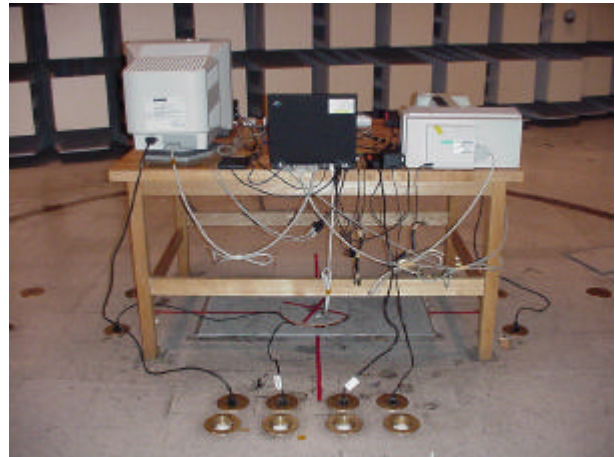
ThinkPad T30 (M/T 2366) Radiated measurement setup photo Rear view
