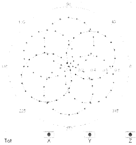
f=600 MHz,TEM
