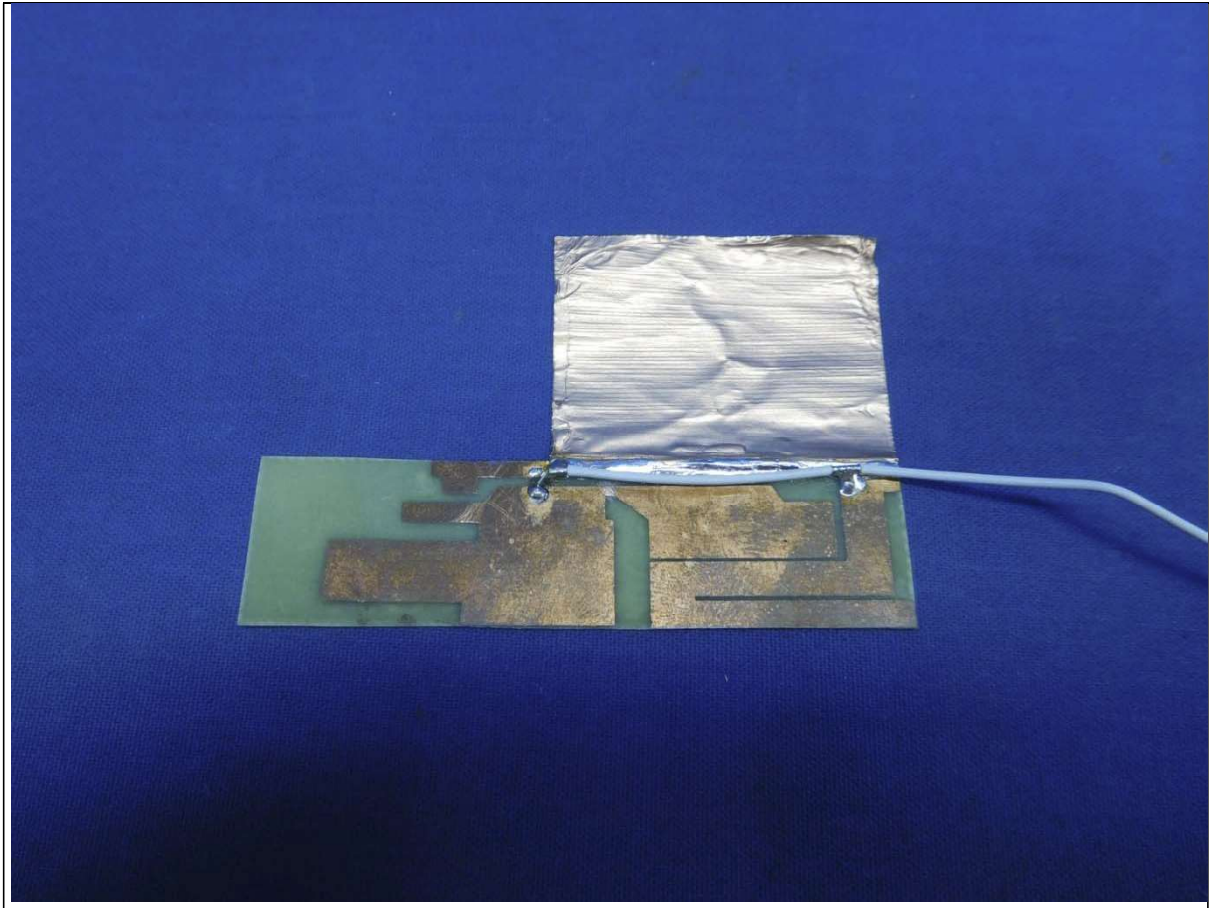
Antenna No. 3
