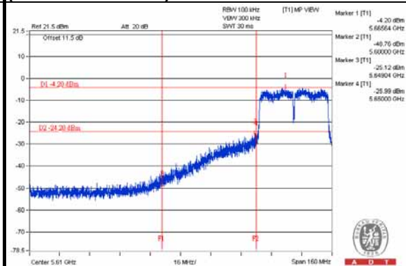
802.11ac (VHT40) OFDM MODULATION (CH 134: 5670MHz)
