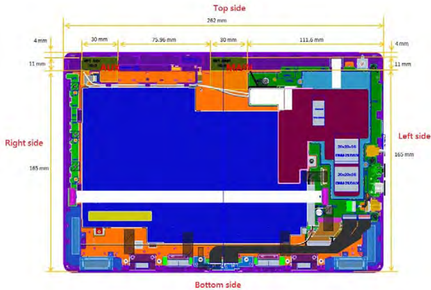
Fig.8 Antenna position of EUT (Back view)
