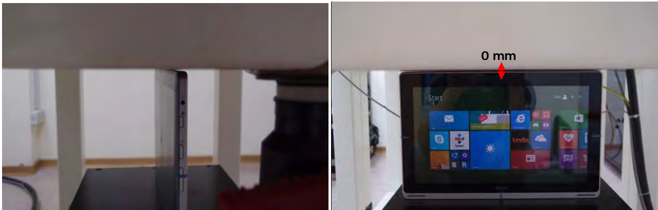
Fig.4 EUT Top side to flat phantom
