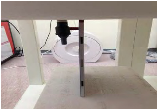
Fig.5 EUT Left side to flat phantom
