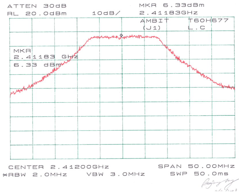
Plots of Peak Output Power for 802.11 g (15.247)
