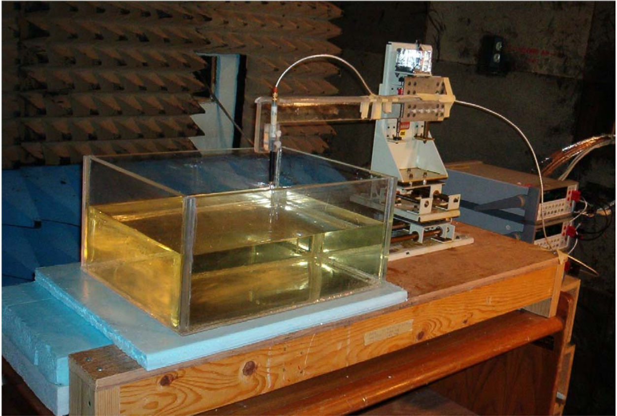
Fig. 6. Photograph of the three-dimensional stepper-motor-controlled SAR measurement system using a planar phantom.
