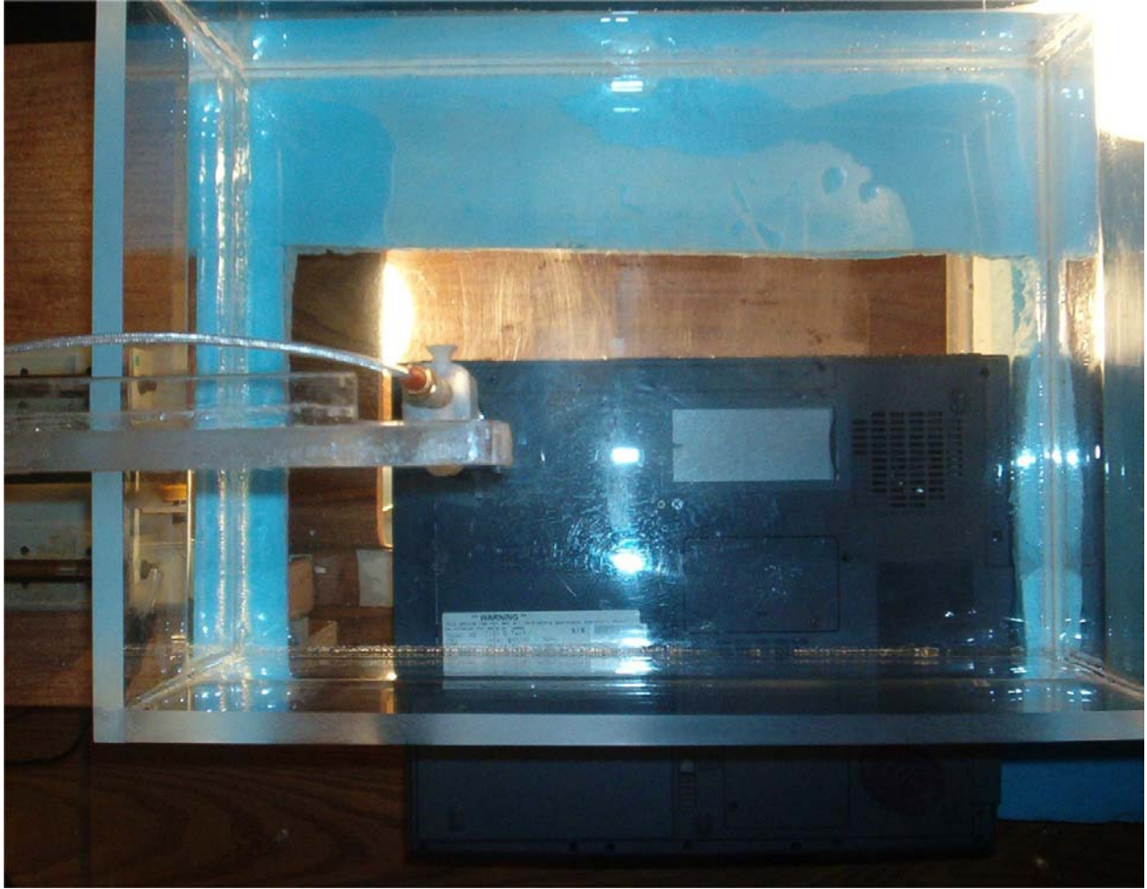
Fig. 4a. Photograph of the bottom of the Acer TravelMate 660 Notebook Computer pressed against the base of the planar phantom. This is Configuration 1 – Laptop position for SAR testing.
