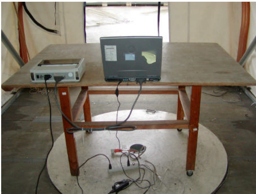
Radiated Emission - Rear View, BY27 Antenna
