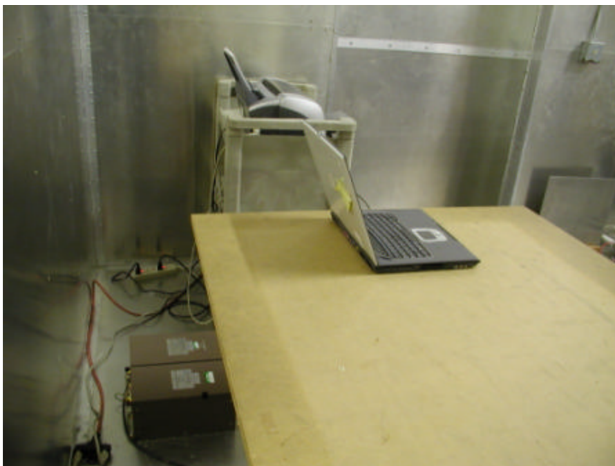
Conducted Emission - Side View, ZIIS Antenna
