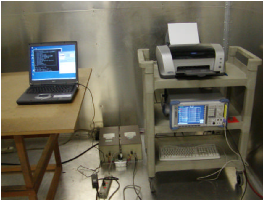
Conducted Emission - Front View, BY27 Antenna
