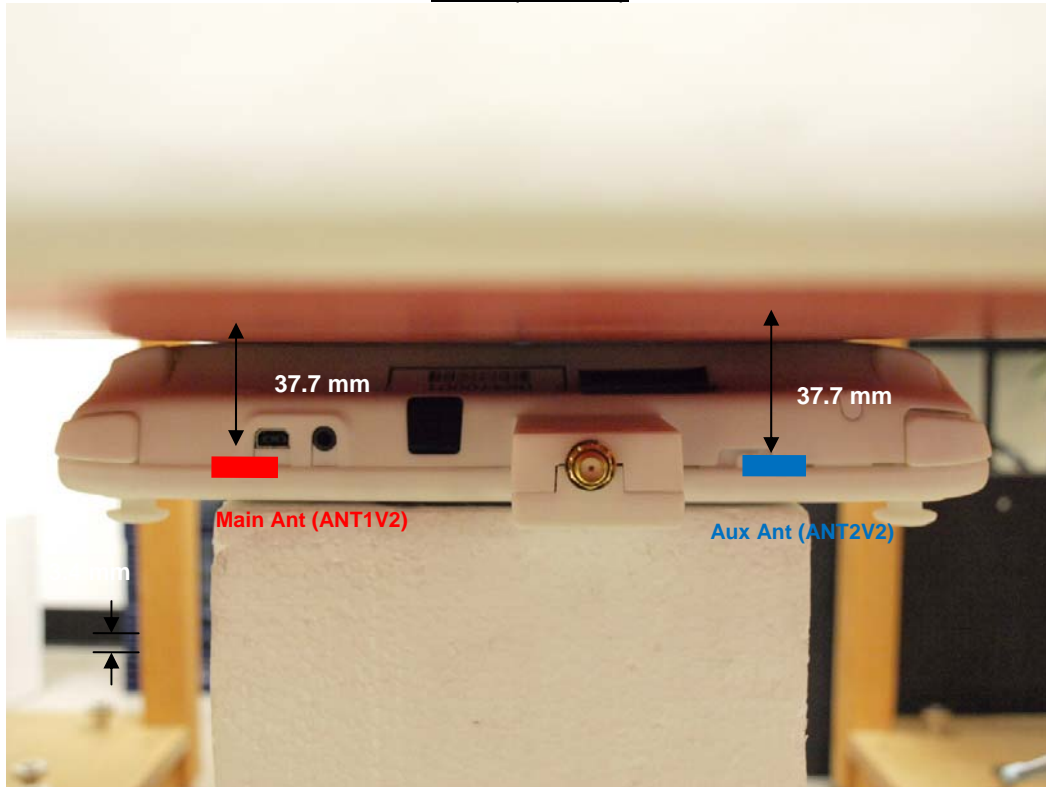
Rear (bottom)
