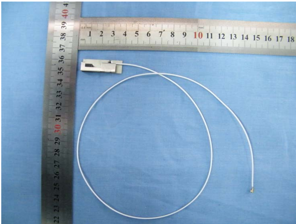
MSA-3411-25GC1-A1-W550MM---Bluetooth Antenna 2 (Cable length is 550mm)
