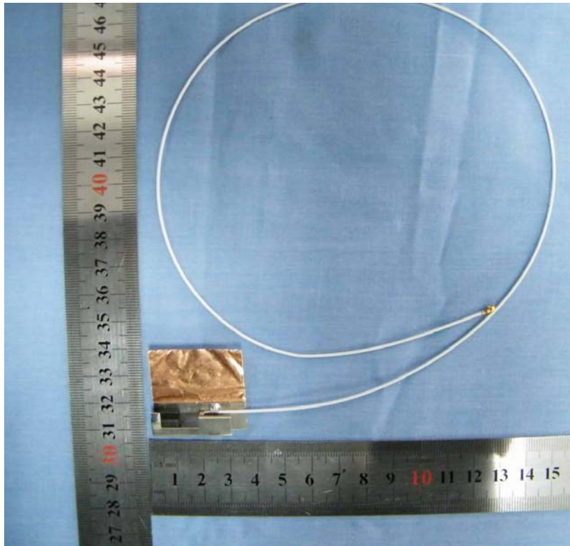
MSA-3411-25GC1-A1-W550MU---Bluetooth Antenna 1 (Cable length is 550mm)
