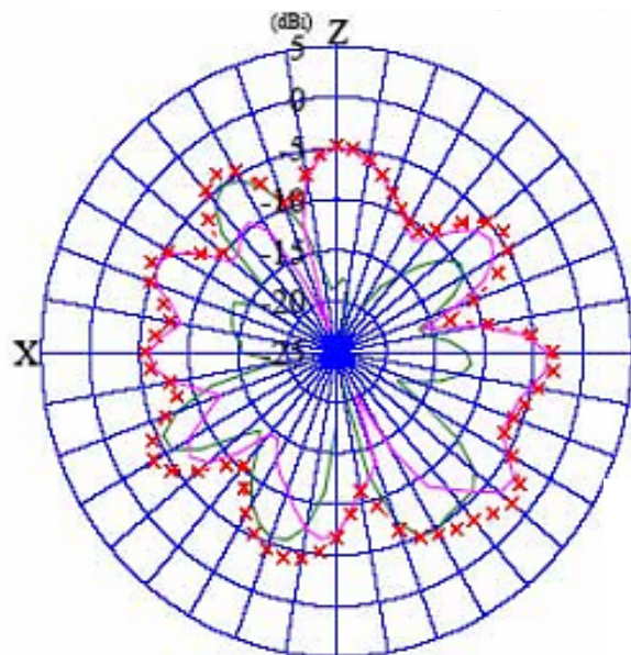
Vertical Radiation Pattern (Passive)
