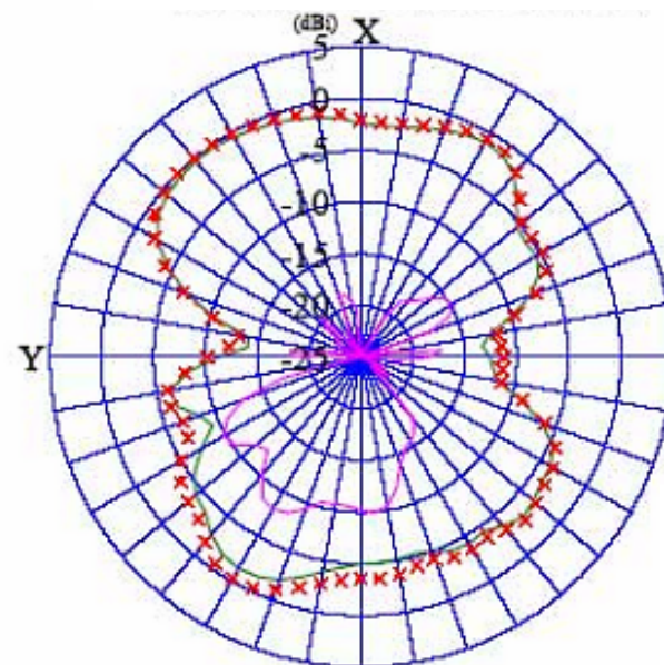
Vertical Radiation Pattern (Passive)
