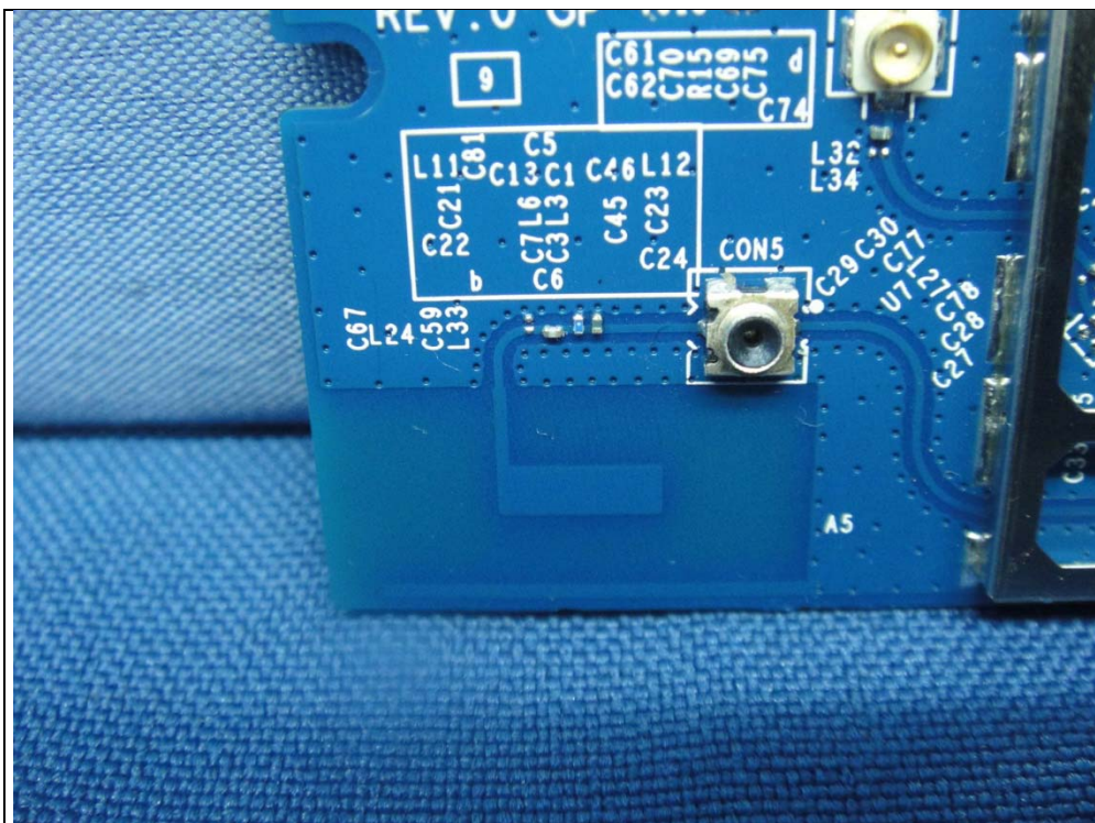
For WLAN used antenna (Model No.: J20H086)
