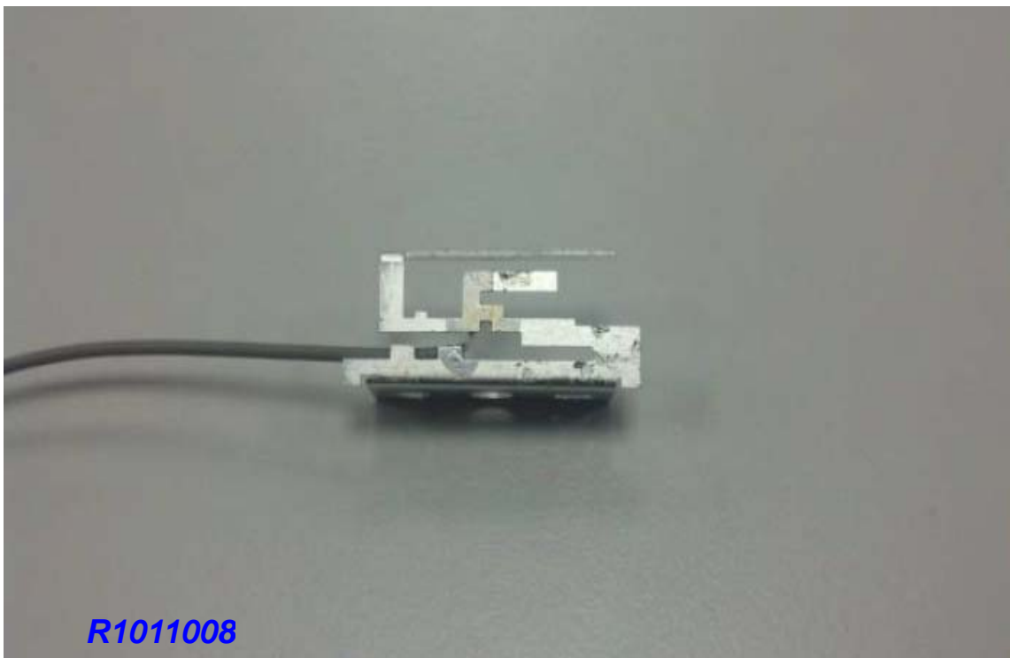
Ant.10: WDAN-1PCVT007-1F
