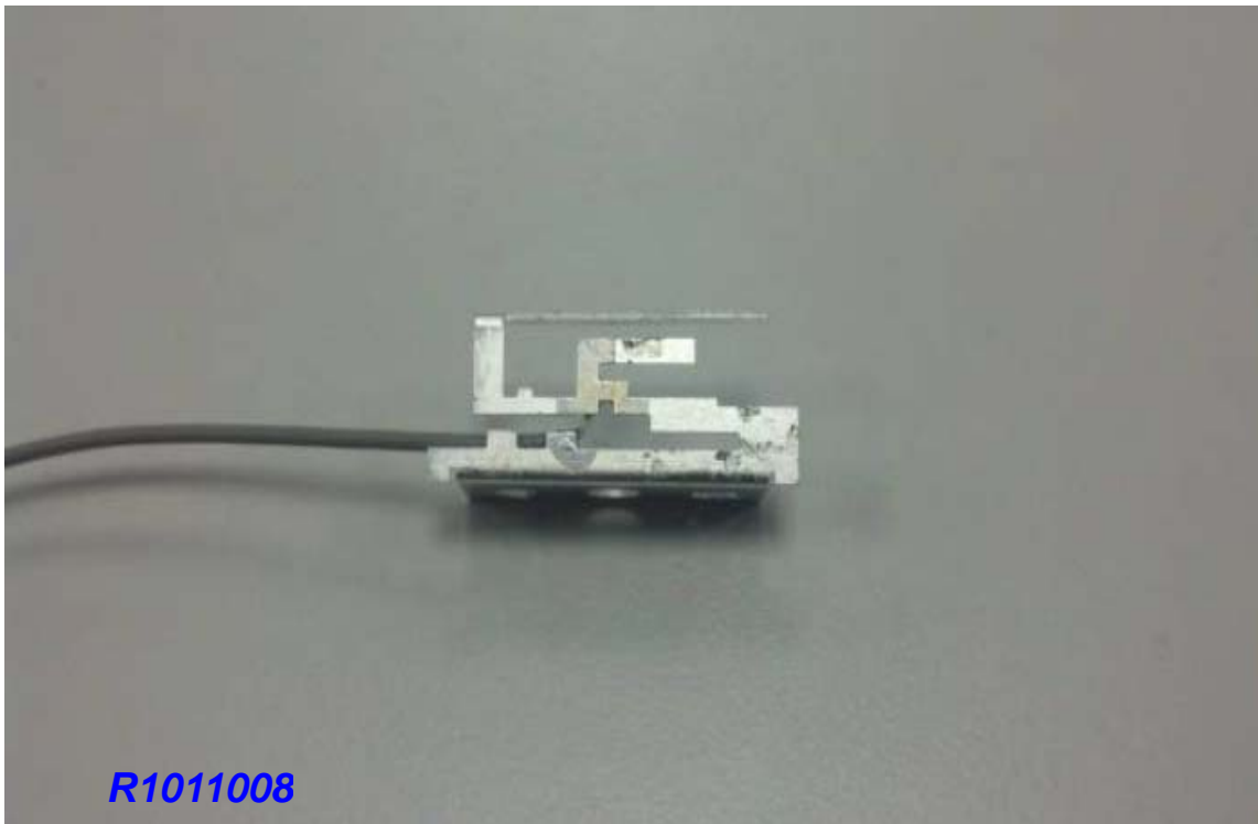
Ant.5: WDAN-1PCVT004-1F
