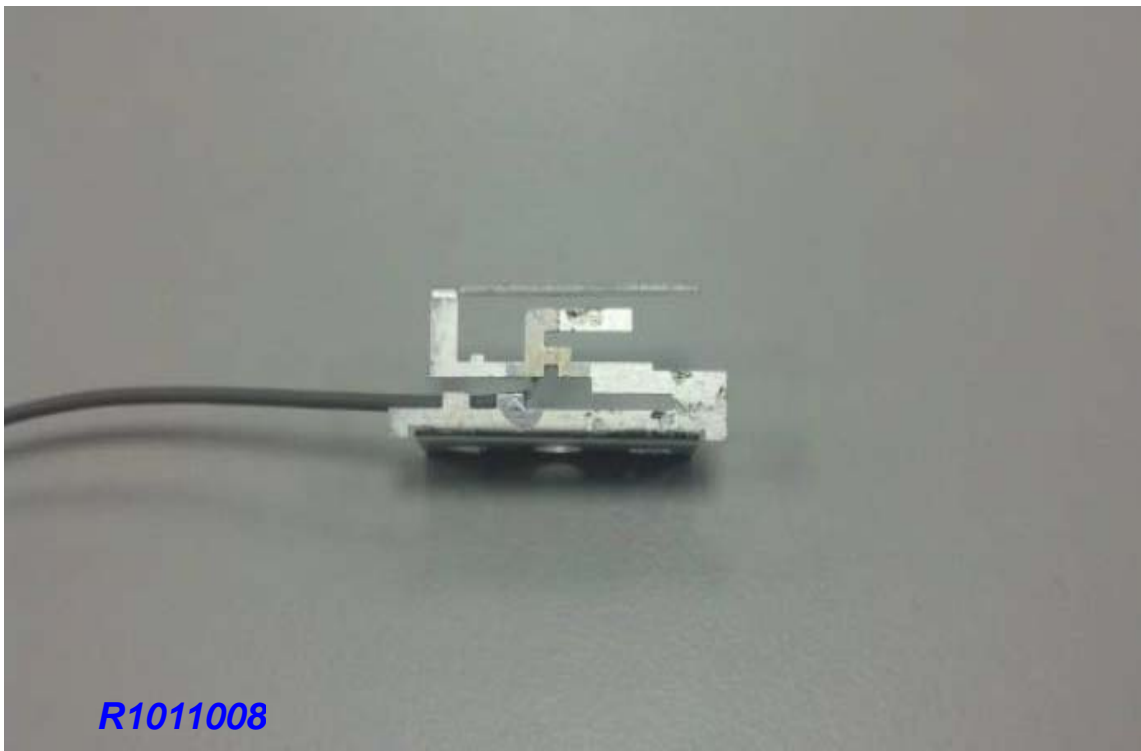
Ant.6: WDAN-1PCVT004-1F
