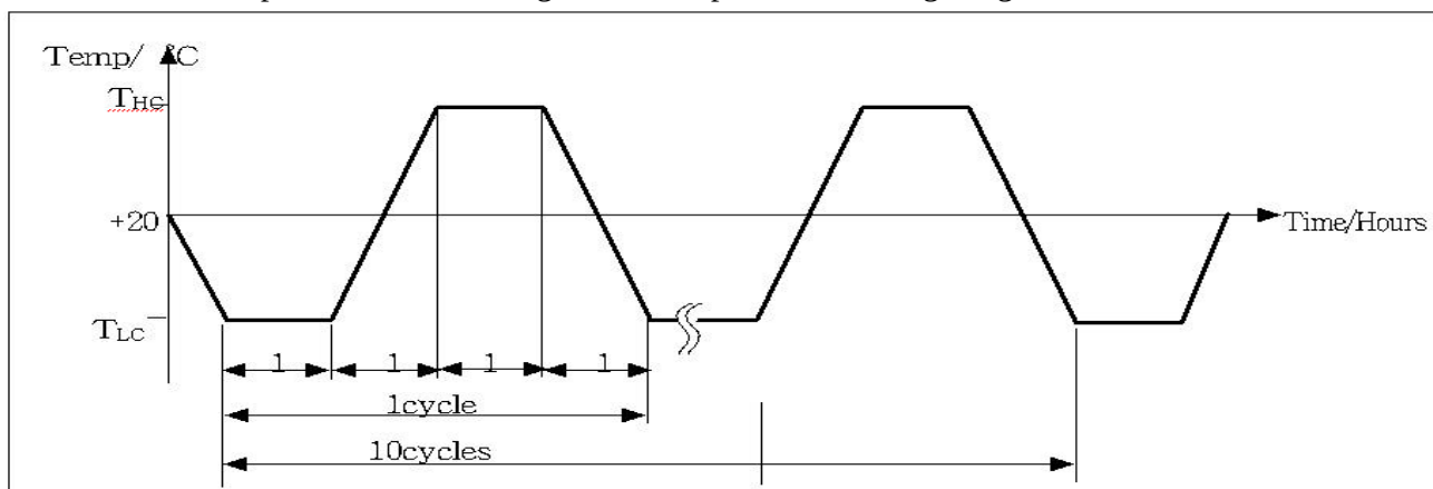
Figure 4.2.4. Temperature cycling.
