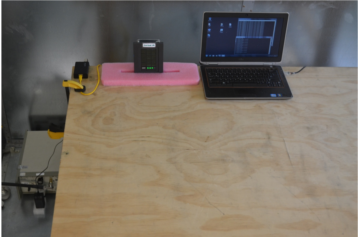
Conducted Emissions
