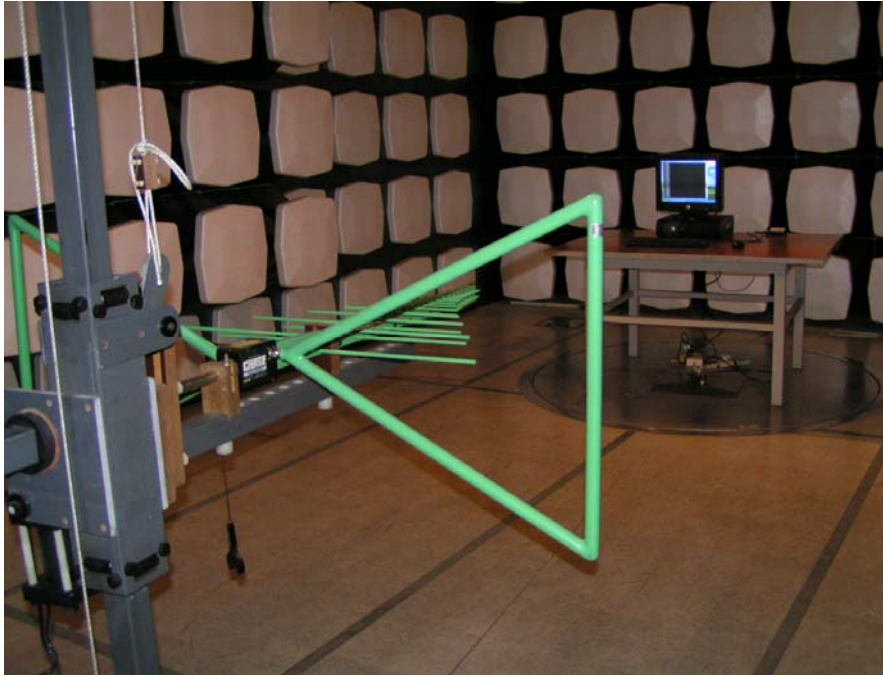
Field Strength Test Set-up - Front View
