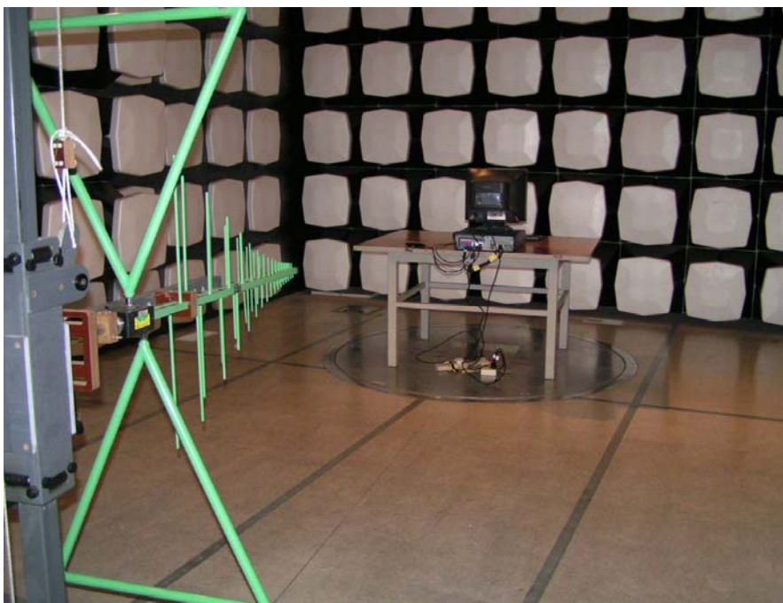
Field Strength Set-up - Rear View
