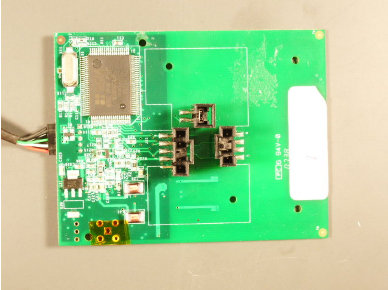
EUT PCB Bottom View – Shield Removed
