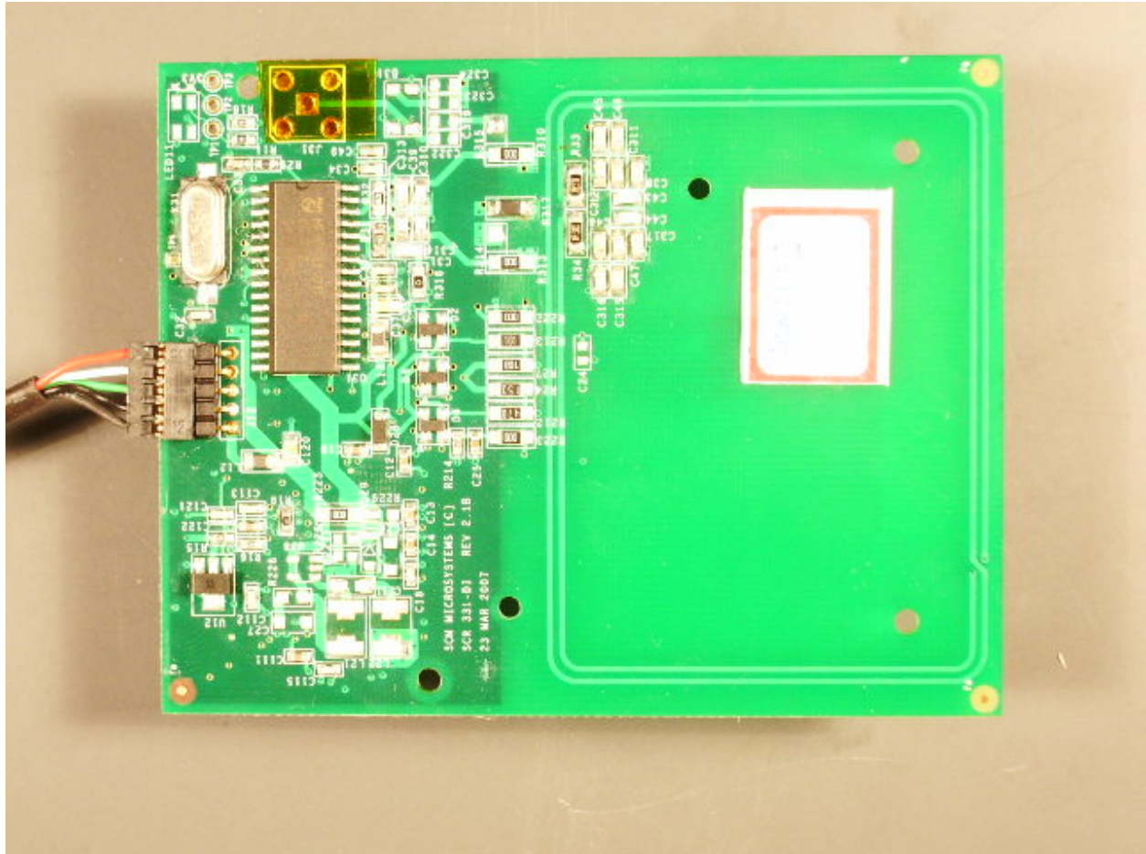
EUT PCB Top View – Shield Removed
