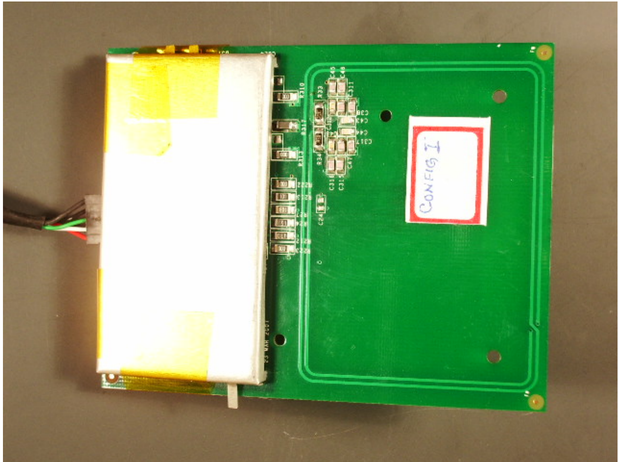
EUT PCB with shield Top View
