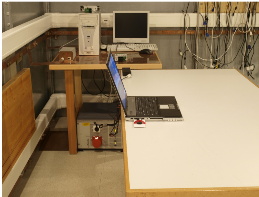
Picture 6: Setup in shielded room for conducted emission test setup
