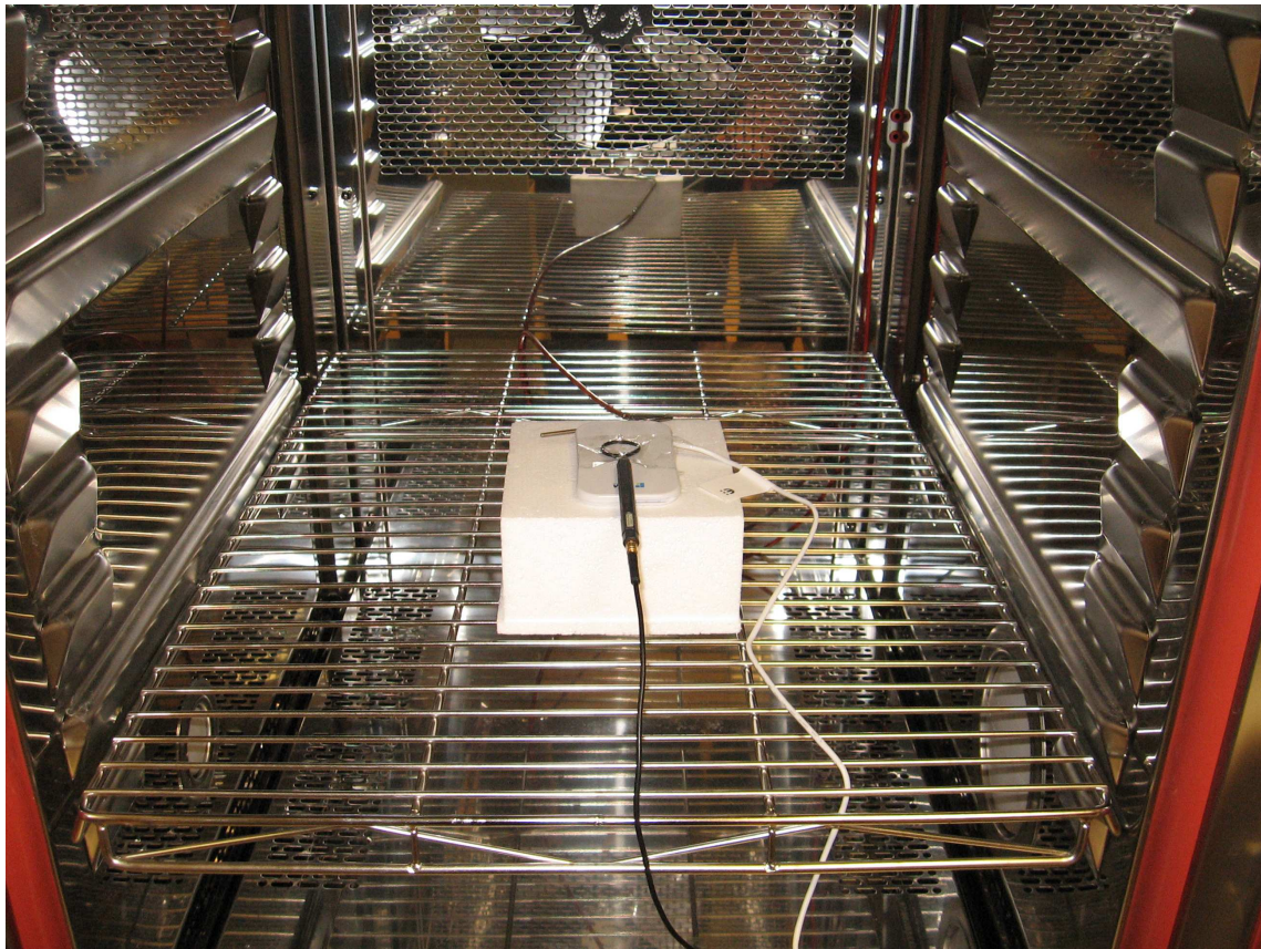
Picture 7: Carrier frequency stability test setup
