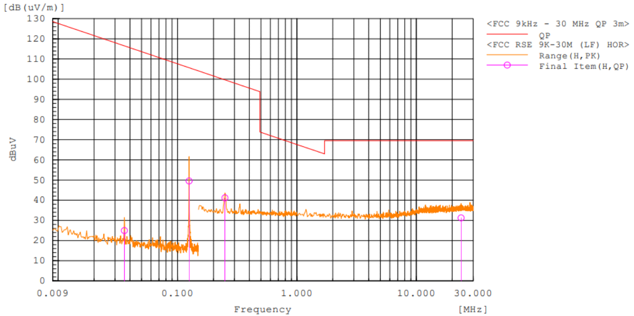
Radiated Spurious Emission 9 kHz – 30 MHz (Antenna Position 180°) : LF FSK
