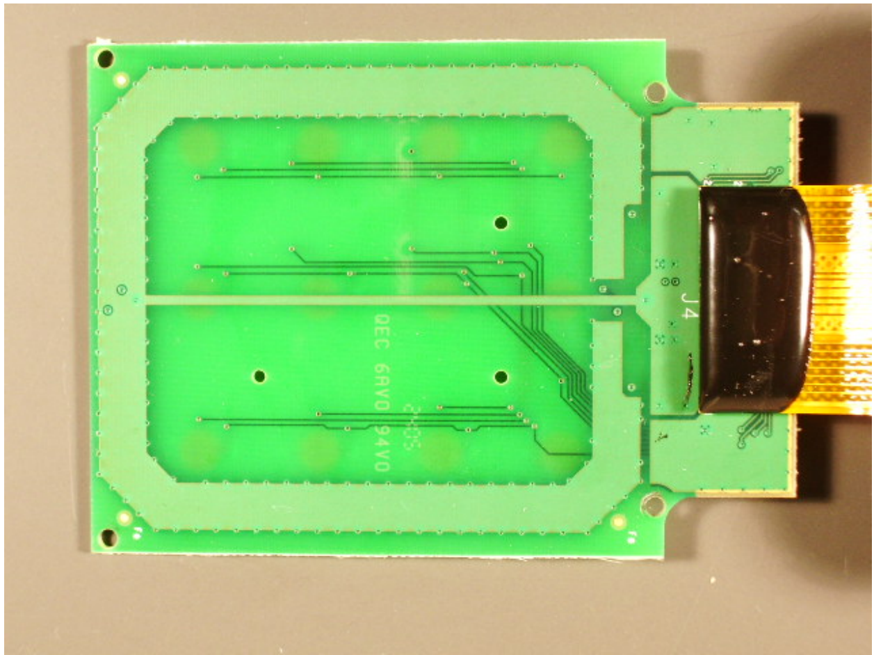
Antenna PCB – Bottom View
