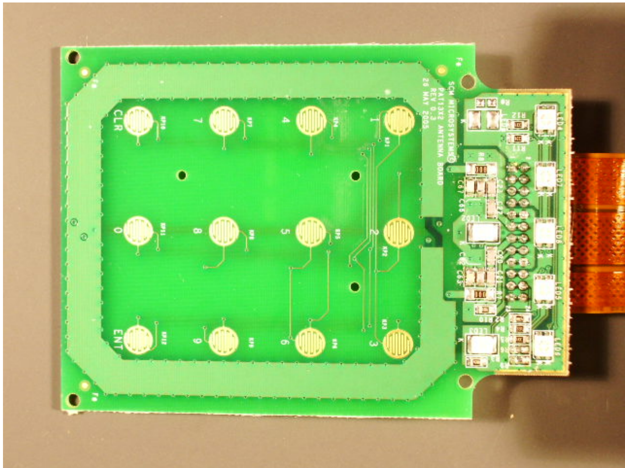
Antenna PCB – Top View
