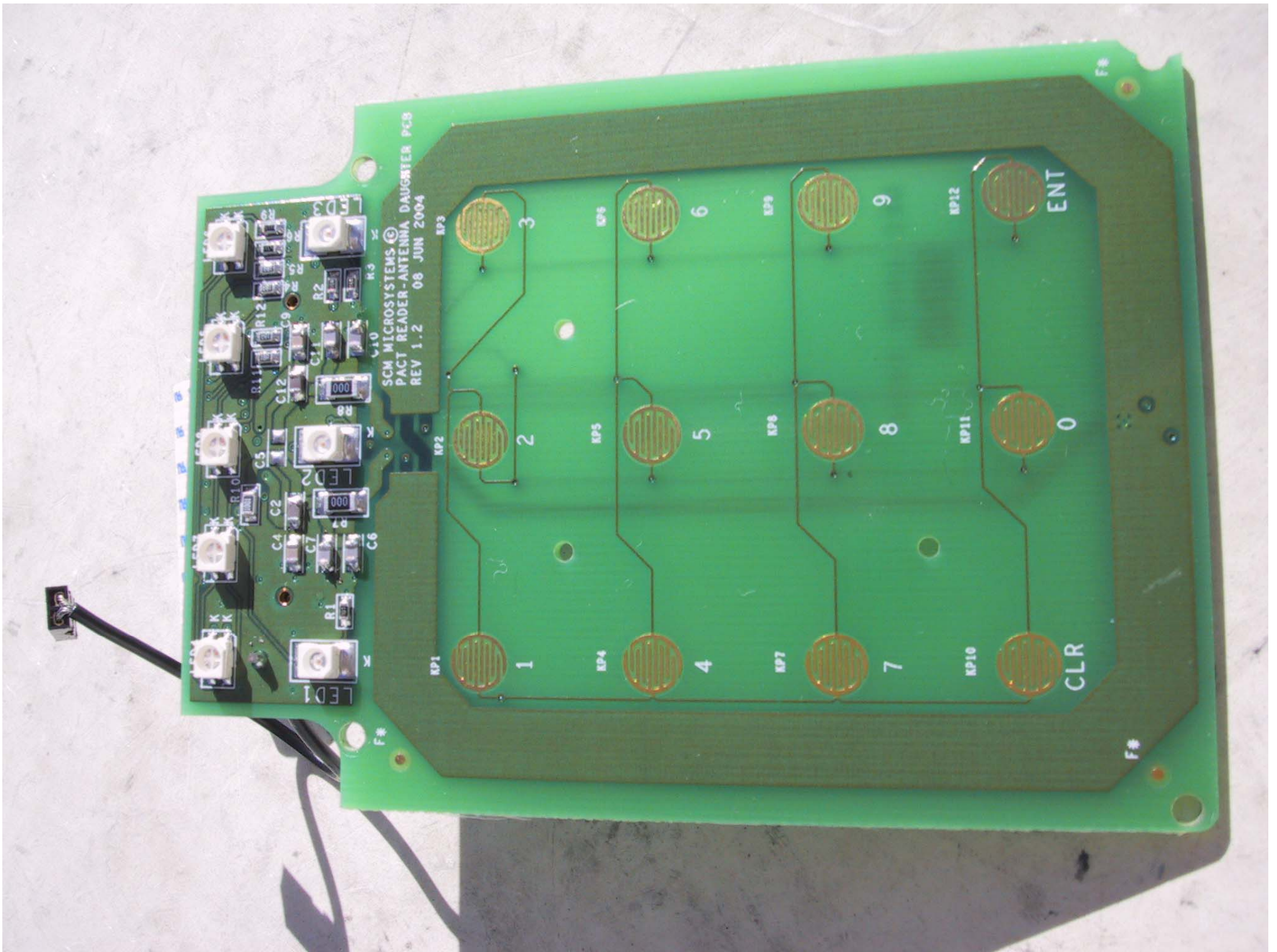
Antenna Daughtercard – Sensors
