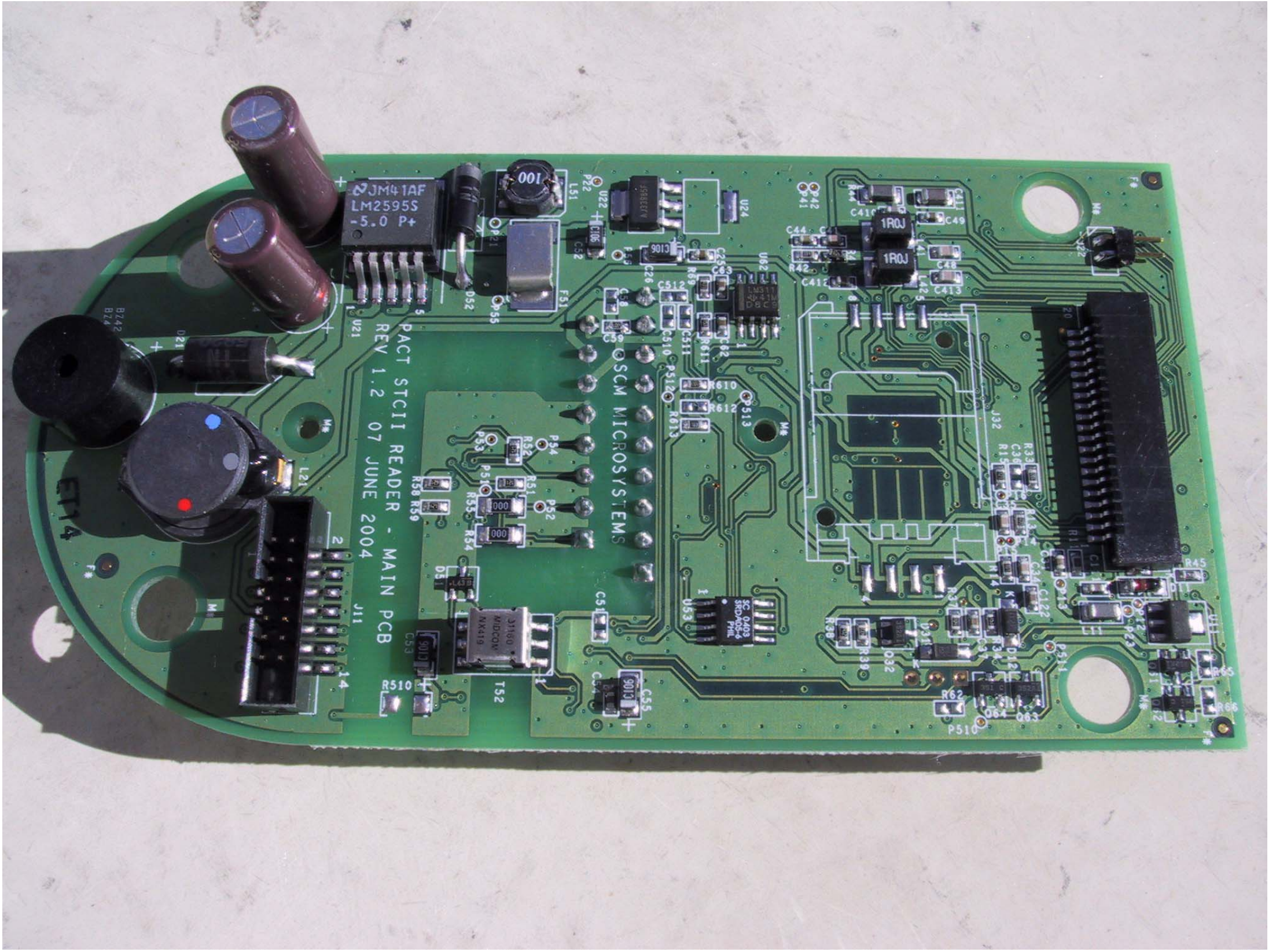
Main PCB – Top
