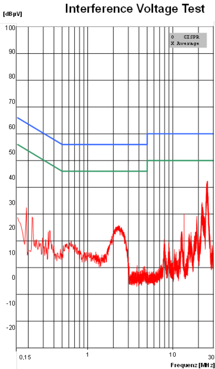
Picture 3: Conducted emission on mains, neutral (Chart),
