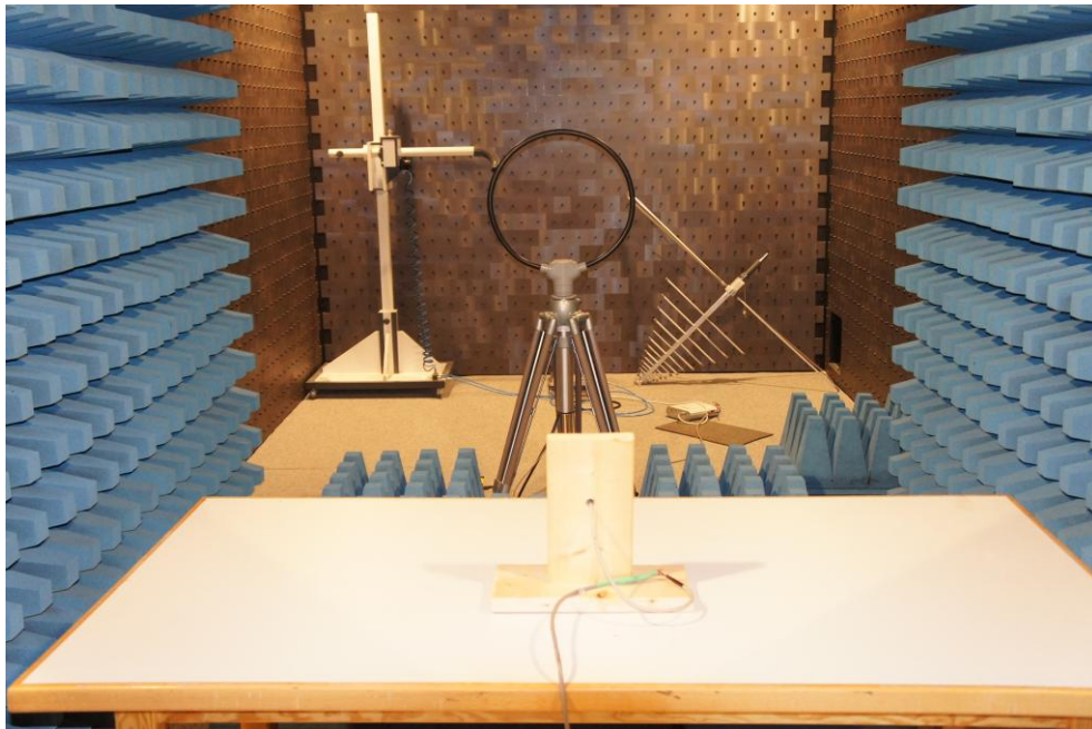
Picture 1: EUT test setup radiated emission test (9kHz to 30MHz)
