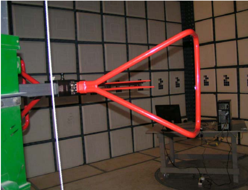
Maximized Radiated Emission Test Set-up - Front View
