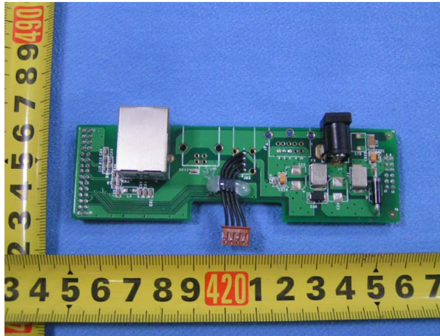
LAN and Power Connector Board Front View
