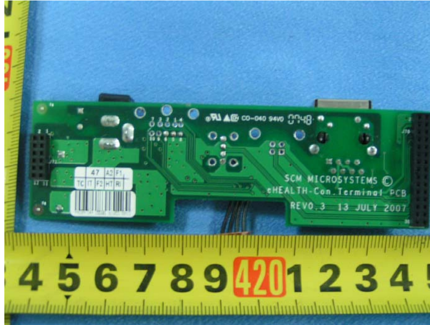
LAN and Power Connector Board Rear View
