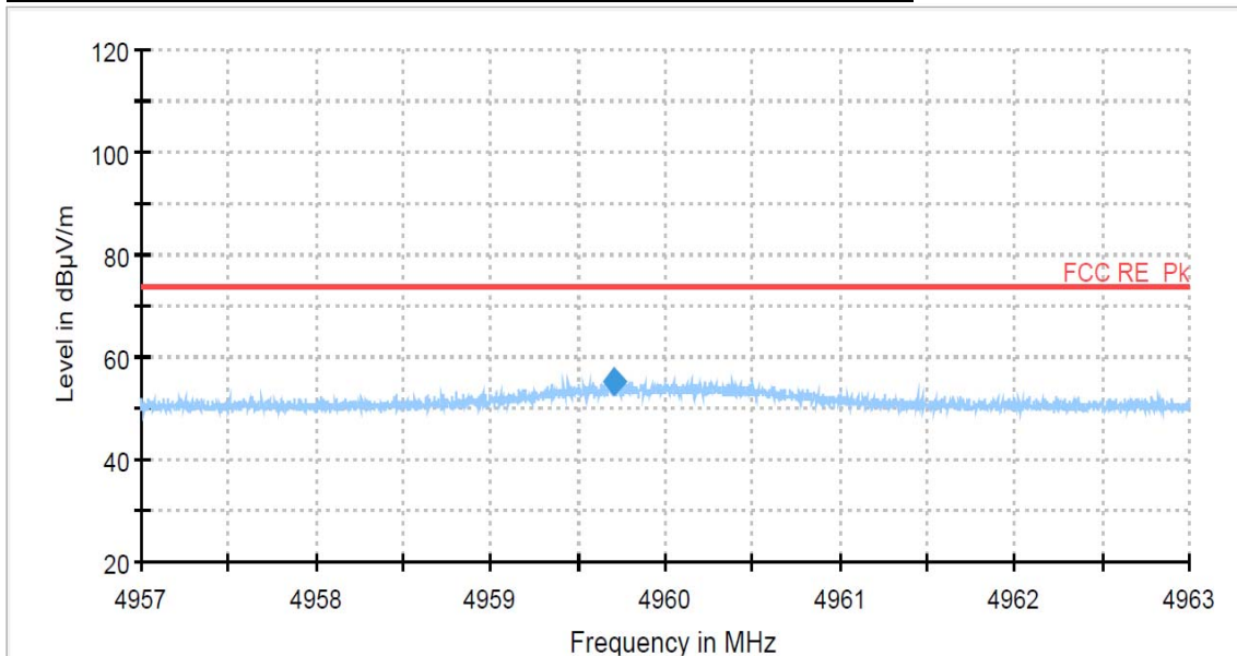
Worst Case : 2480 MHz GFSK modulation : 2 nd Harmonic Pk
