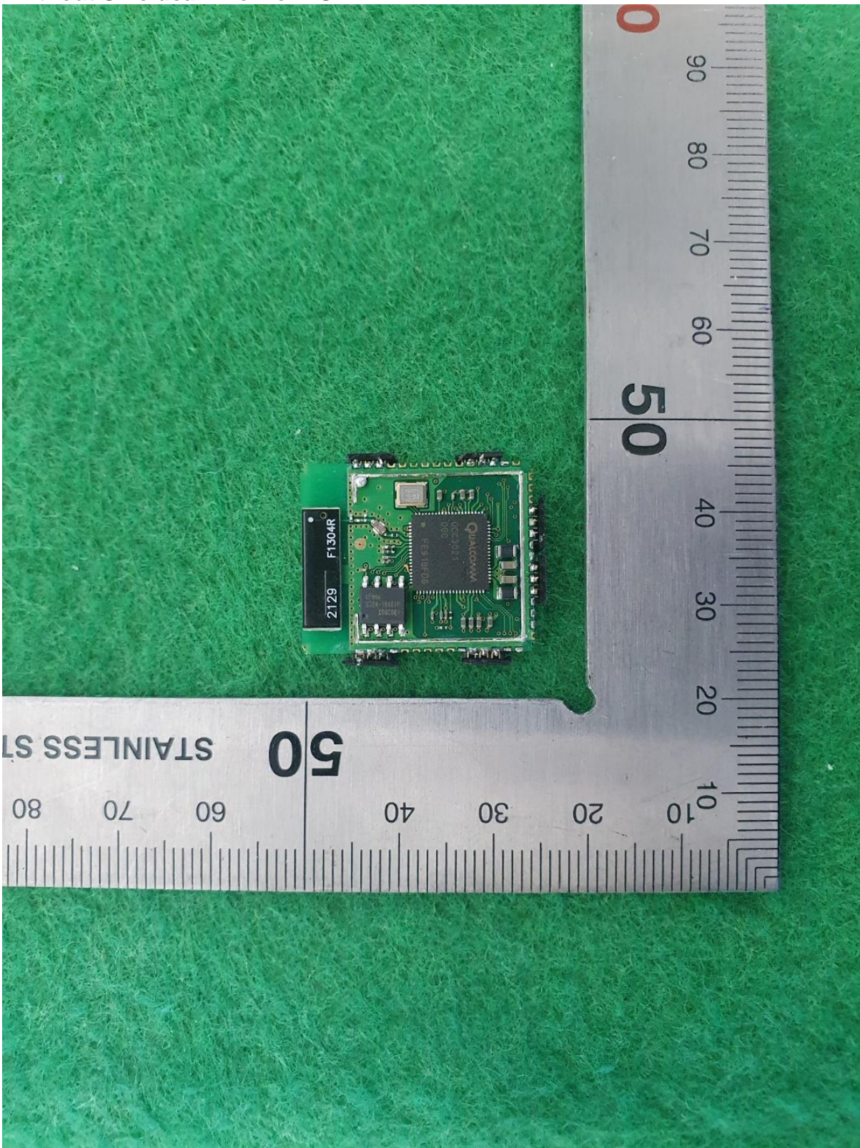
Without Shieldcan View of EUT
