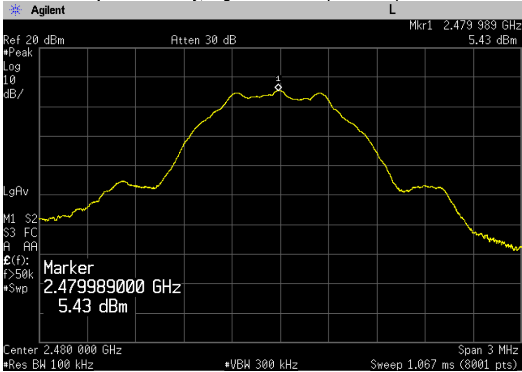
Peak Power Spectral Density, Highest Channel (2480 MHz)
