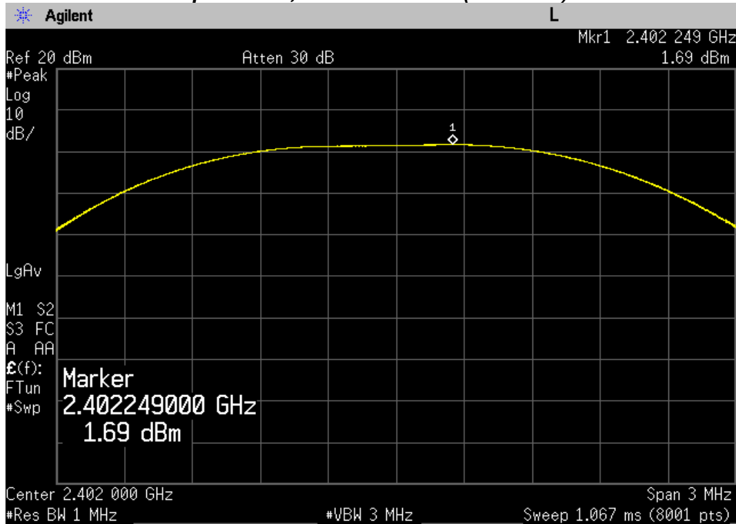
Maximum Peak Output Power, Lowest Channel (2402 MHz)
