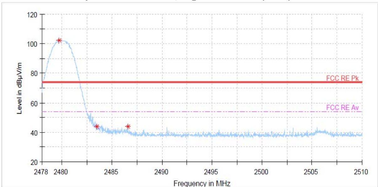
Restricted Band Spurious Emissions, Highest channel (Peak)
