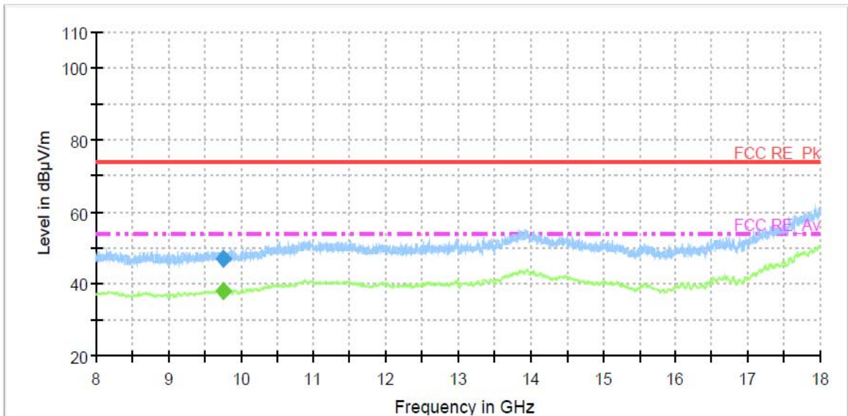
Worst Case : 2442 MHz GFSK modulation : 8 GHz to 18 GHz
