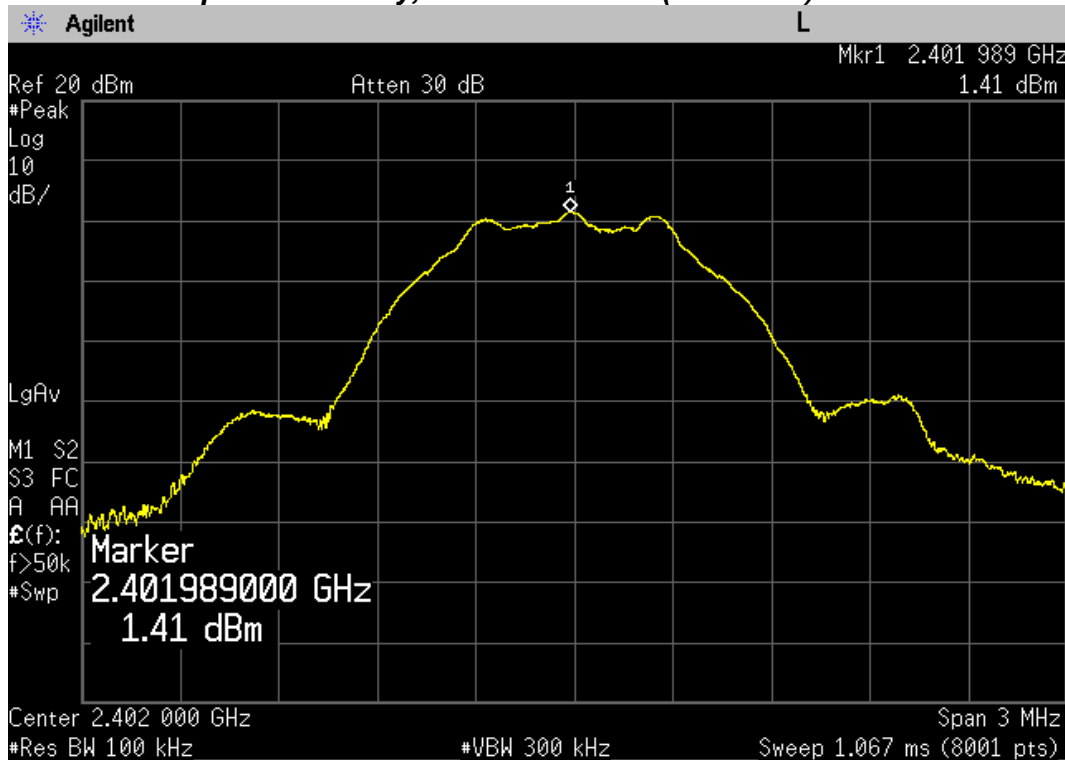
Peak Power Spectral Density, Lowest Channel (2402 MHz)
