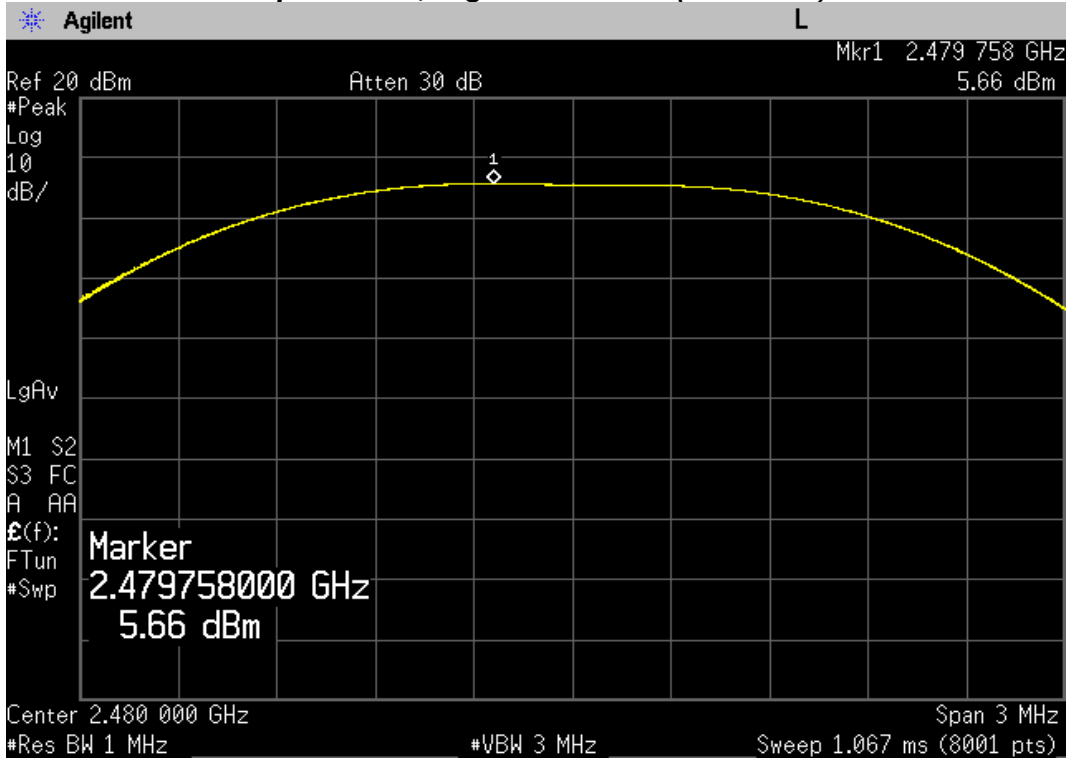
Maximum Peak Output Power, Highest Channel (2480 MHz)
