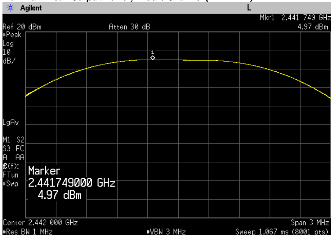
Maximum Peak Output Power, Middle Channel (2442 MHz)
