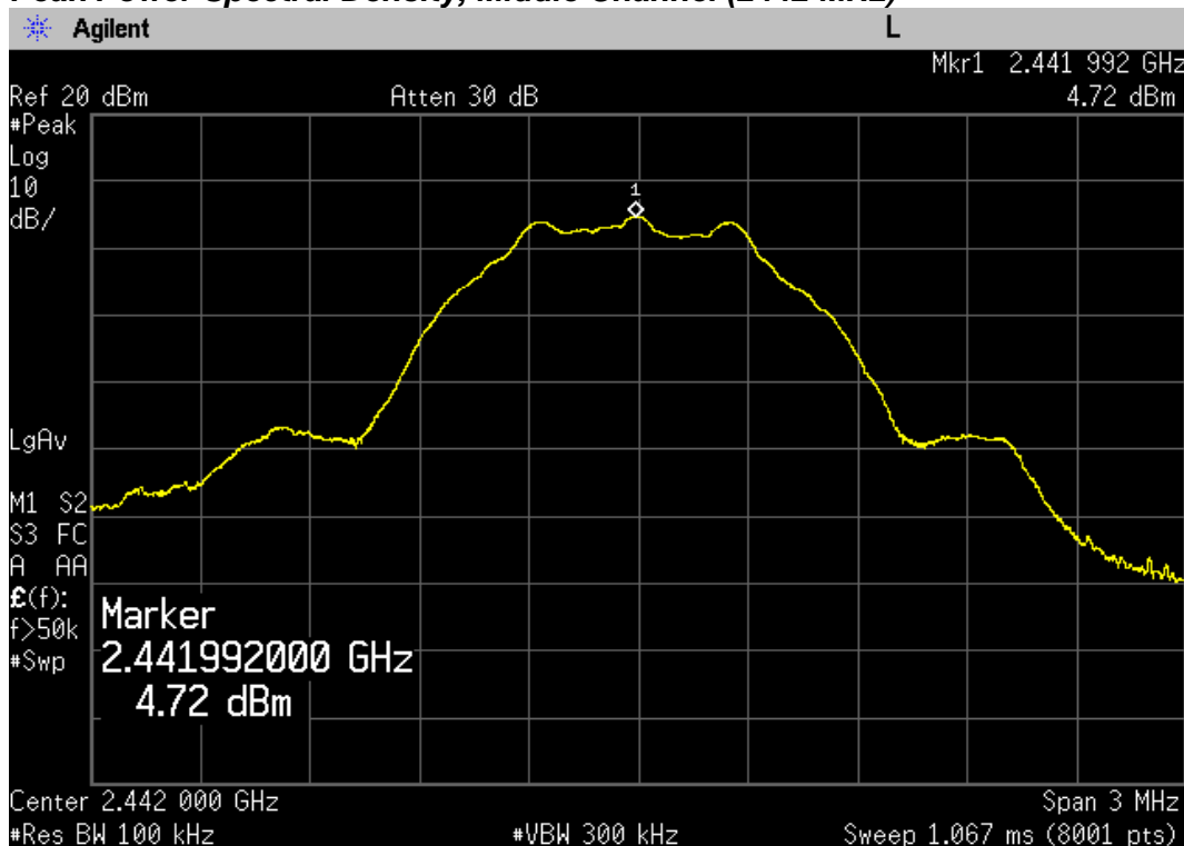
Peak Power Spectral Density, Middle Channel (2442 MHz)
