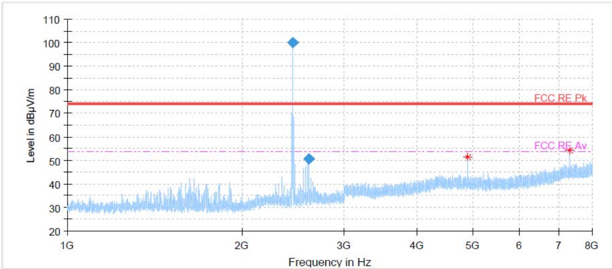
Worst Case : 2442 MHz GFSK modulation : 1 GHz to 8 GHz
