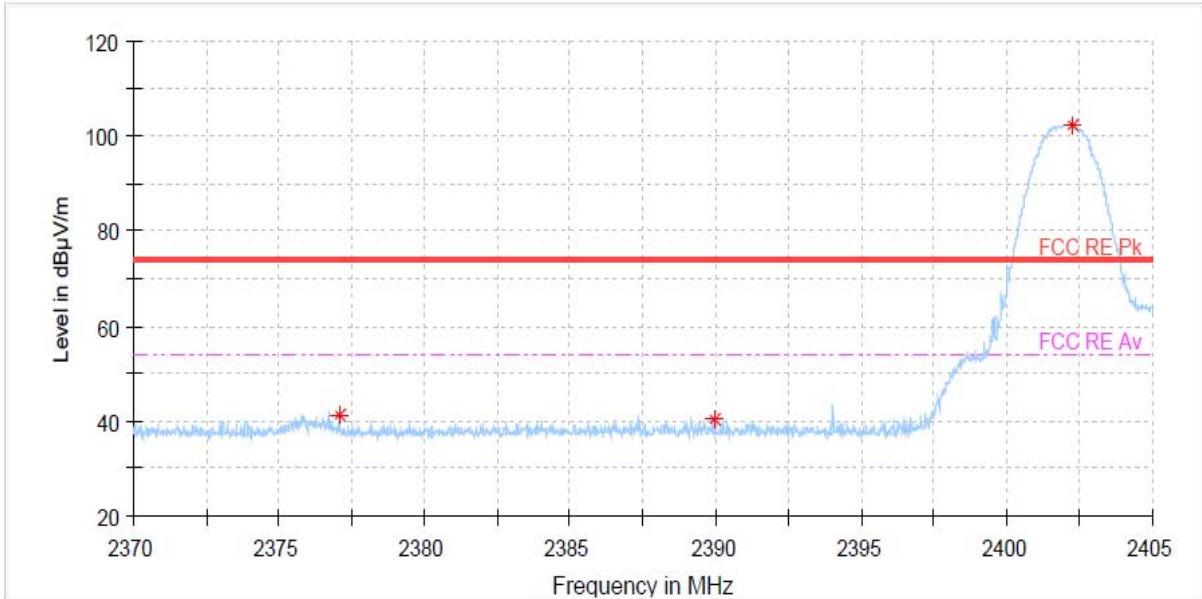
Restricted Band Spurious Emissions, Lowest channel (Peak)
