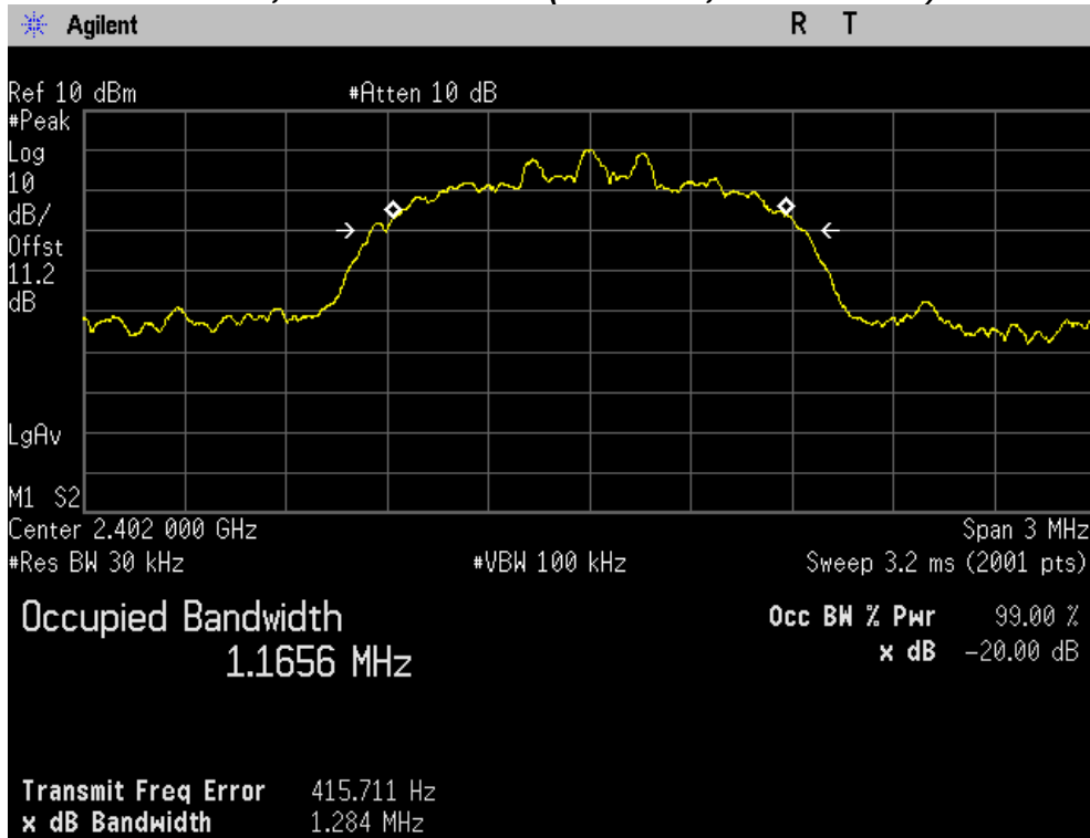
20 dB Bandwidth, Lowest Channel (2402 MHz, 8DPSK Mode)
