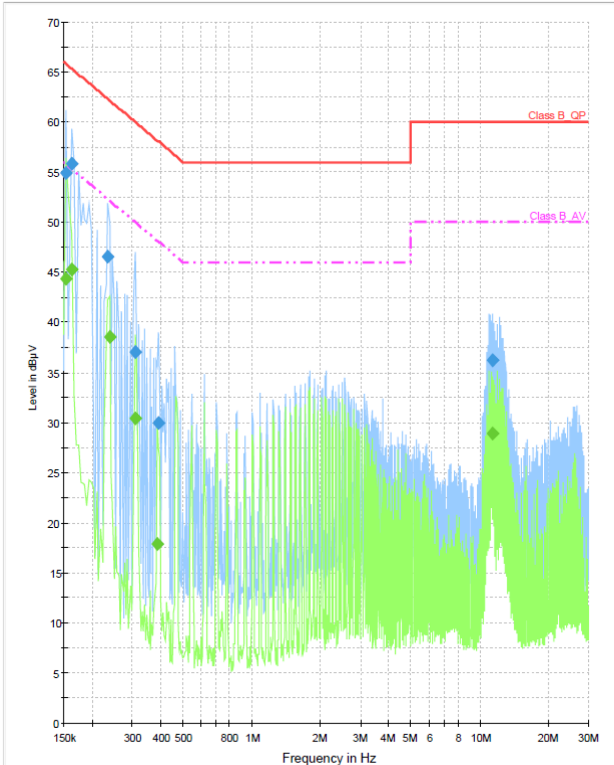
Conducted Emission at the Mains port (Line + Neutral)
