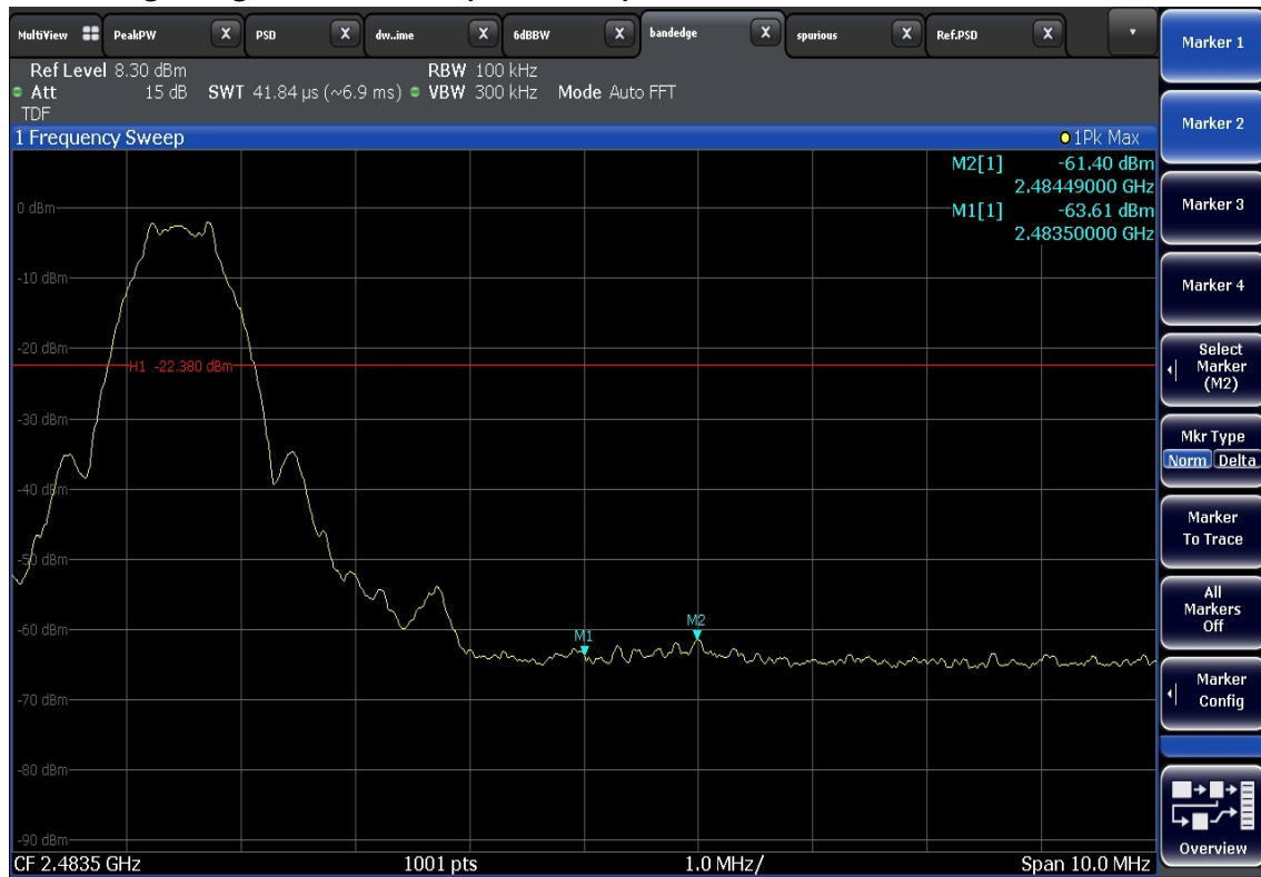
Band Edge, Highest Channel (2480 MHz)
