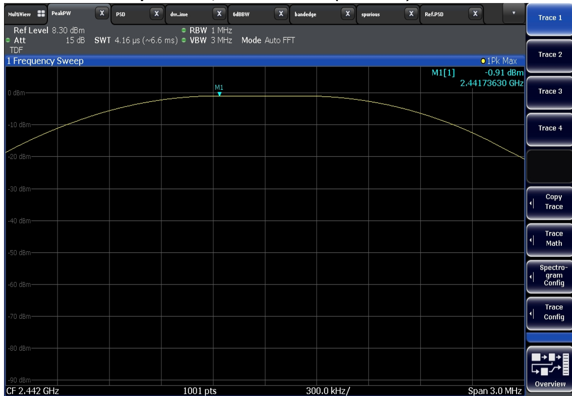
Maximum Peak Output Power, Middle Channel (2442 MHz)
