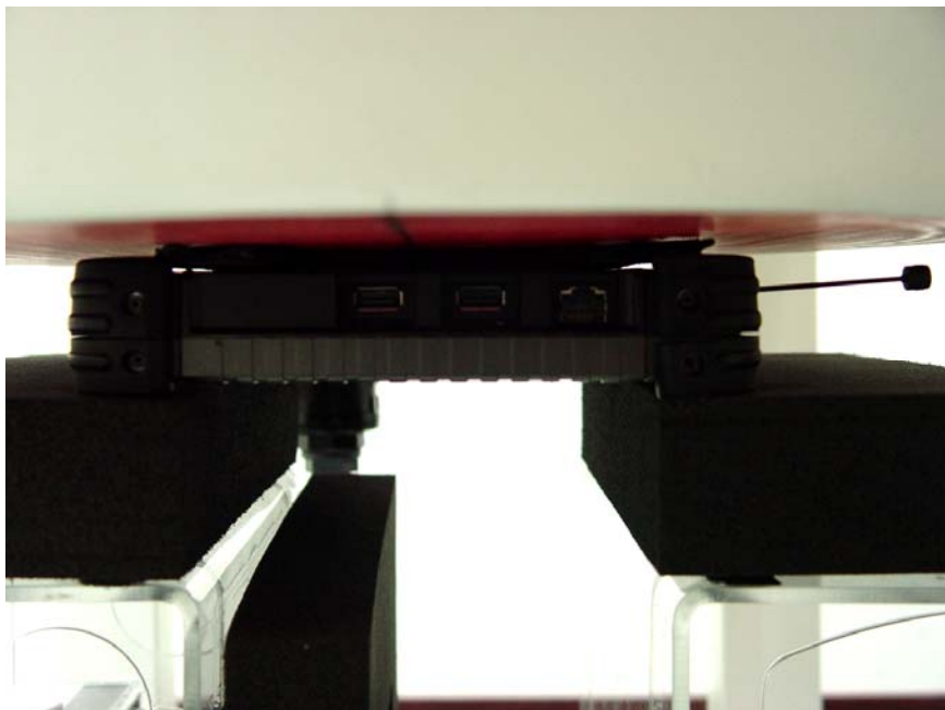
Rear Face with 0 cm Gap with Ant-Extend
