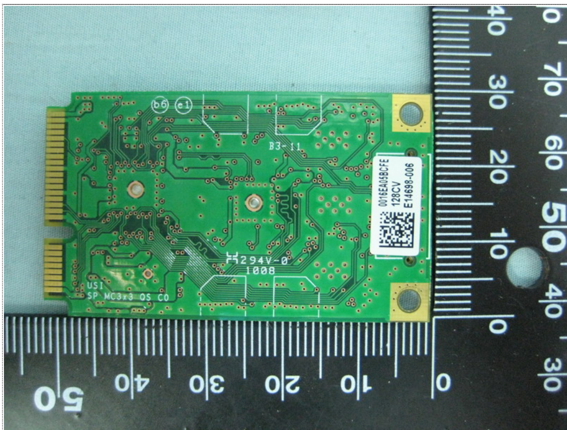
Rear View of EUT-1 (533AN MMW)
