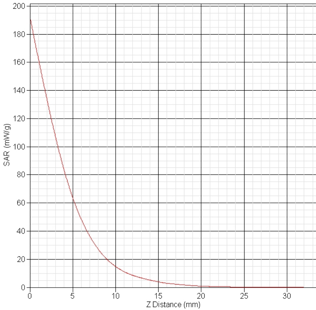
SAR-Z Axis at Hotspot x:0.14 y:-2.01
