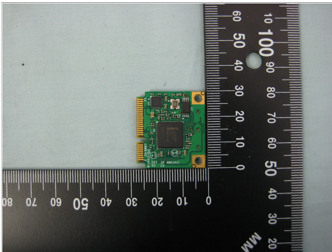
Rear View of EUT-1 (533AN_HMW)
